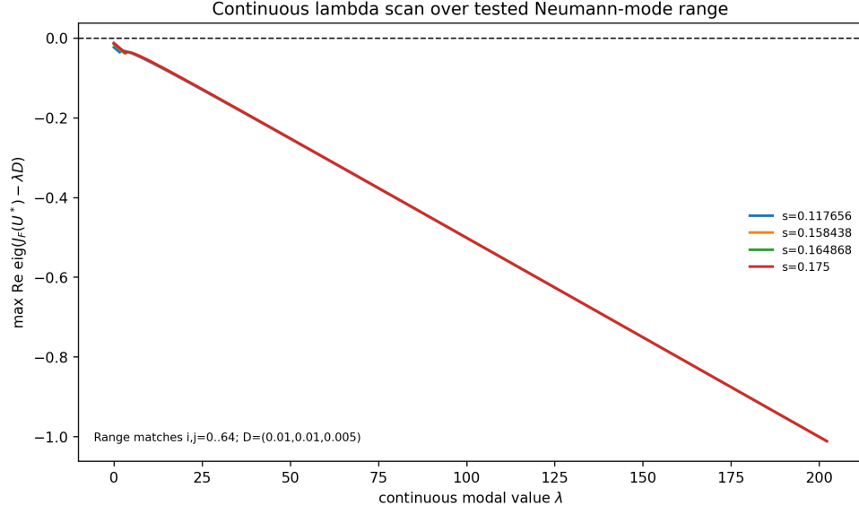
Figure 5: Continuous \lambda -scan for J_F(U^*) - \lambda D over 600 equally spaced \lambda values in the mode-equivalent range corresponding to i, j = 0, \dots, 64 . This scan strengthens the tested spatial-mode result over that range, but it is still a tested-range diagnostic rather than a proof for all possible modes or diffusion coefficients.
