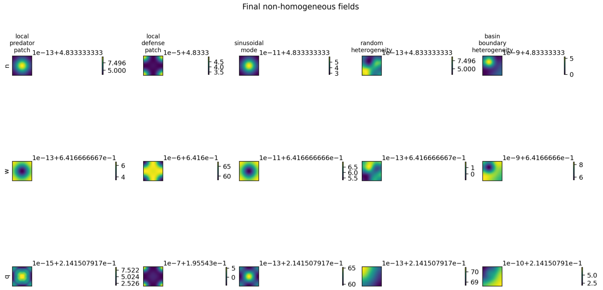
Figure 7: Final PDE fields for representative targeted non-homogeneous perturbation tests. This diagnostic figure supports the absence of persistent spatial patterning in the displayed cases, but it is not a proof for all heterogeneous initial conditions.
