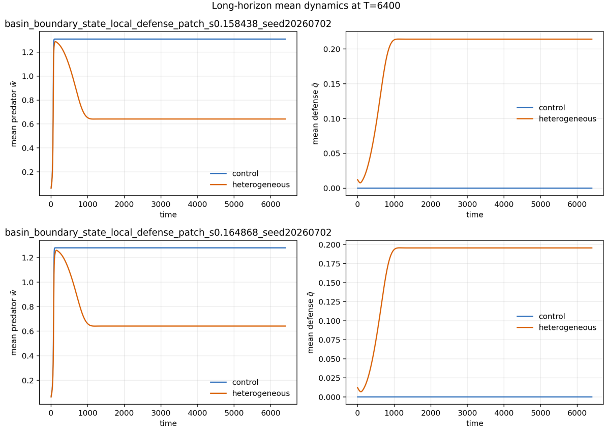
Figure 10: Long-horizon mean time series for the finite-horizon basin-changing non-homogeneous cases. The followed cases are the targeted cases selected from the earlier finite-amplitude tests, not a broad PDE scan.
