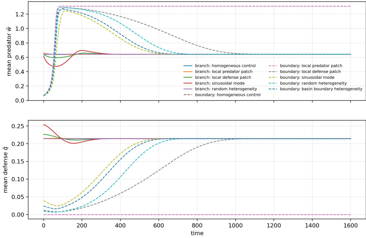
Figure 8: Mean dynamics for targeted finite-amplitude non-homogeneous PDE tests. These diagnostic trajectories support comparison with matched homogeneous controls; they do not establish global basin behavior.
