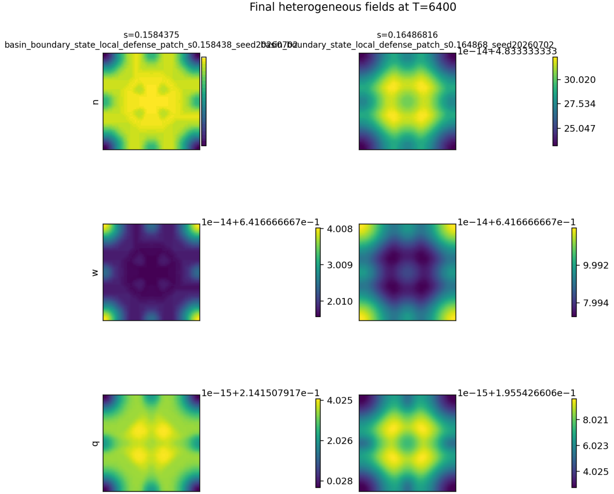
Figure 12: Long-horizon final fields for the followed basin-changing cases. These diagnostics support resolution without persistent spatial patterning for the followed cases.
