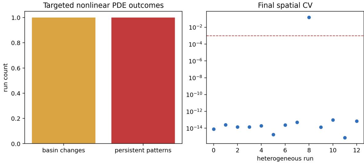
Figure 16: Selected nonlinear non-homogeneous PDE diagnostics. This supporting figure reports targeted finite-amplitude checks for selected nonlinear branches and does not establish global robustness to heterogeneous initial conditions.
