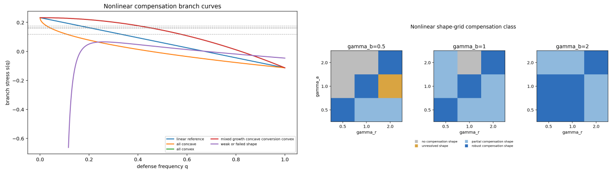
Figure 13: Nonlinear branch curves and shape-grid summary. These figures support selected non-linear compensation branches within the controlled grid.
