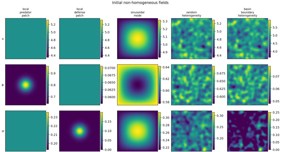
Figure 6: Representative non-homogeneous initial PDE fields for targeted finite-amplitude perturbations. This diagnostic figure documents the tested perturbation classes and is not an exhaustive set of heterogeneous initial conditions.
