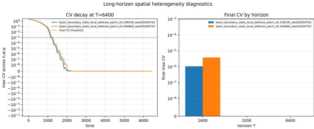
Figure 11: Long-horizon spatial heterogeneity metrics for the followed basin-changing cases. These diagnostics support spatial-pattern decay in the followed cases.
