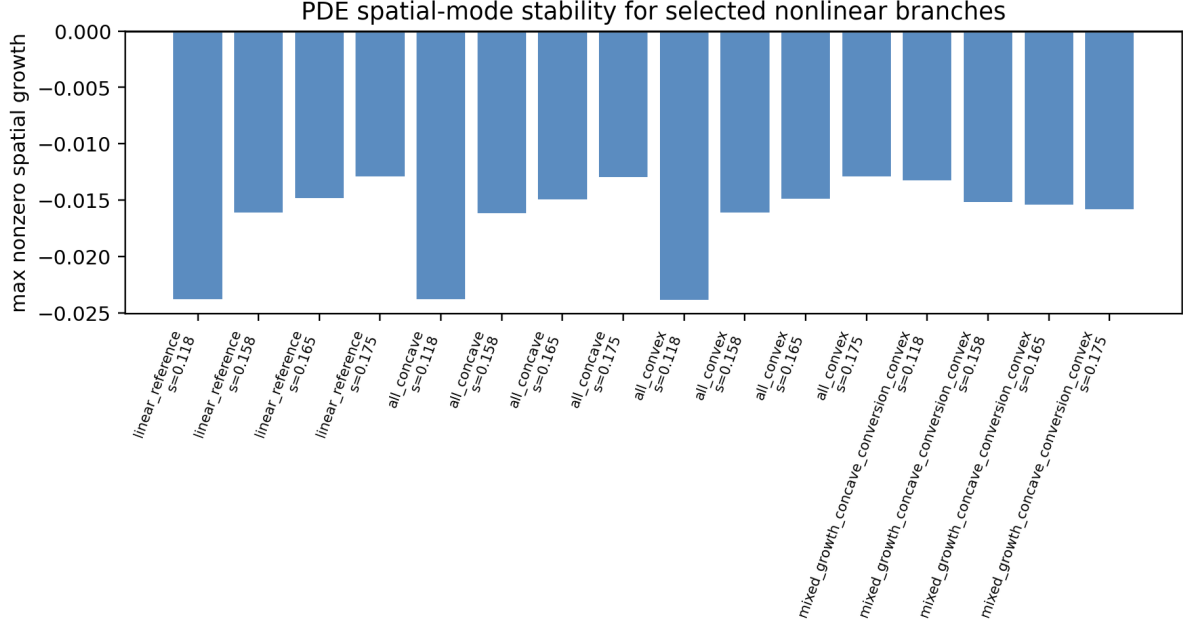
Figure 15: Selected nonlinear PDE spatial-stability diagnostics. This supporting figure reports targeted spatial-stability checks for selected nonlinear branches and does not prove stability for all nonlinear trade-off shapes.
