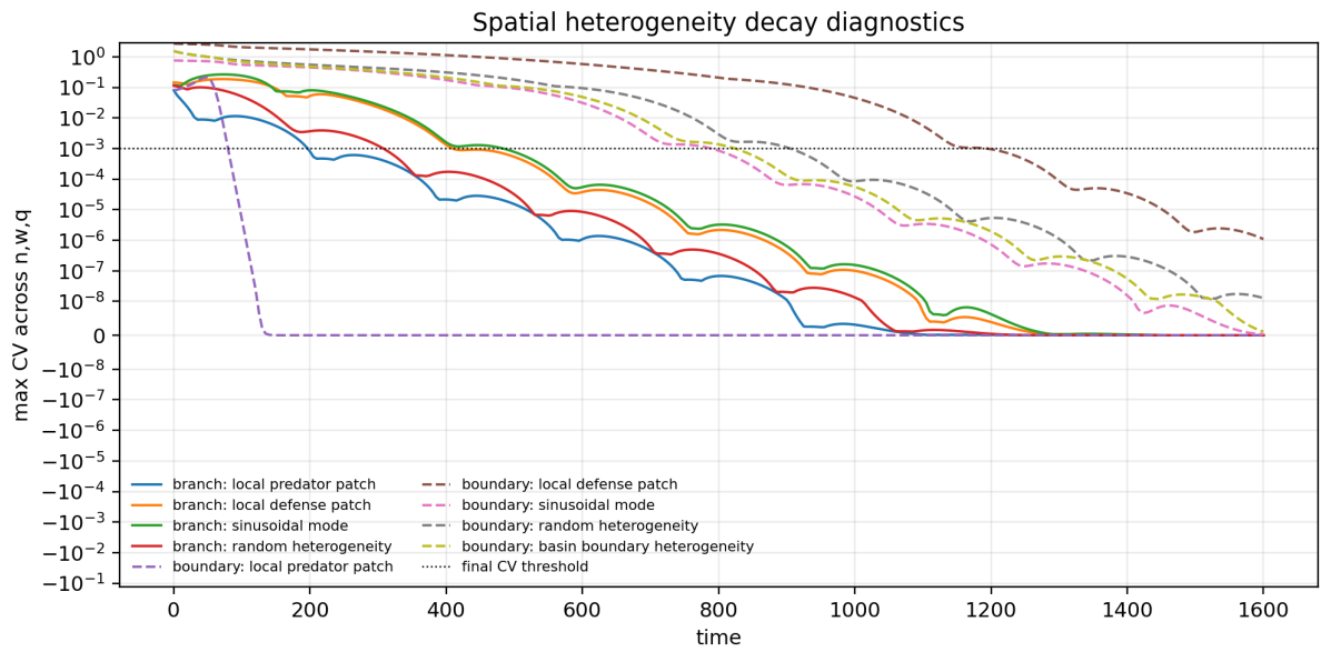
Figure 9: Spatial coefficient-of-variation diagnostics for targeted finite-amplitude non-homogeneous PDE tests. These diagnostics track heterogeneity decay in the tested runs and are not a theorem for all finite-amplitude perturbations.
