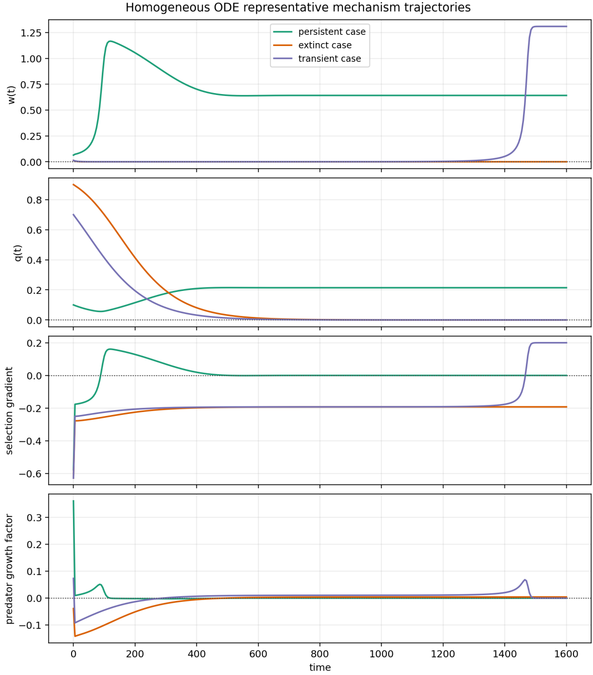
Figure 15: Representative homogeneous ODE trajectories for predator density w , defense frequency q , selection gradient, and predator growth factor. The cases use the same initial means as the representative PDE comparisons.
