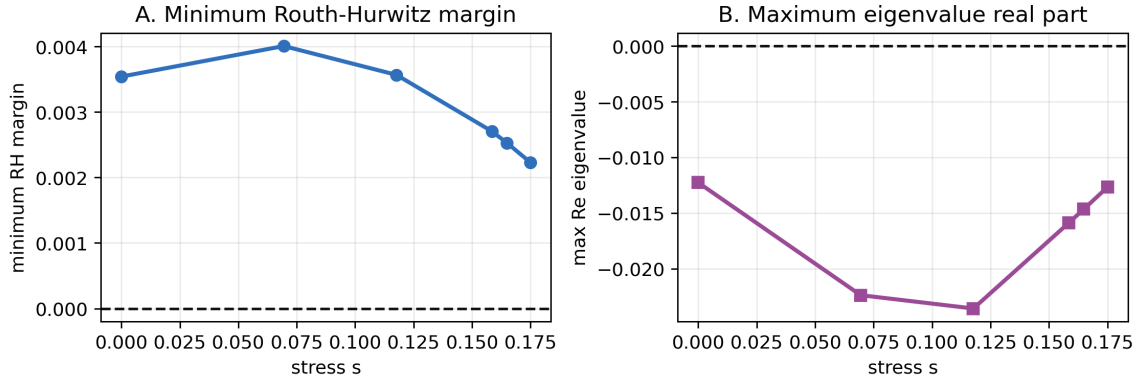
Figure 3: Local stability margins along the compensation branch. Panel A shows the minimum Routh–Hurwitz margin across A_1 , A_2 , A_3 , and A_1 A_2 - A_3 . Panel B shows the maximum real part of the reaction-Jacobian eigenvalues. Positive margins and negative eigenvalue real parts support local stability at the tested stresses; they do not establish global basin attraction or rule out other attractors.
