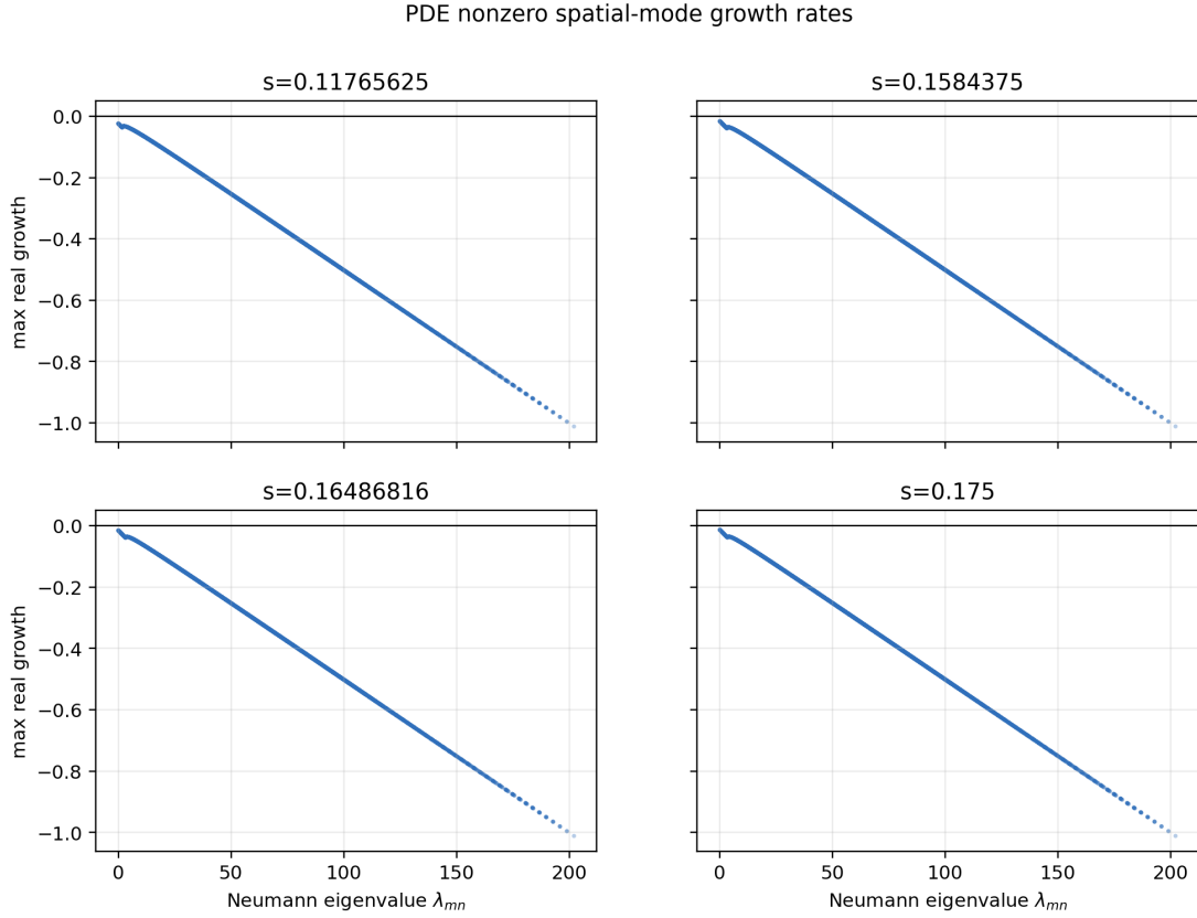
Figure 4: Maximum real growth rates for tested Neumann spatial modes around the homogeneous compensation branch. The figure plots the largest real eigenvalue for modal matrices J_F(U^*) - \lambda_{ij}D . Negative nonzero-mode growth rates support linear spatial stability for the tested diffusion coefficients.
