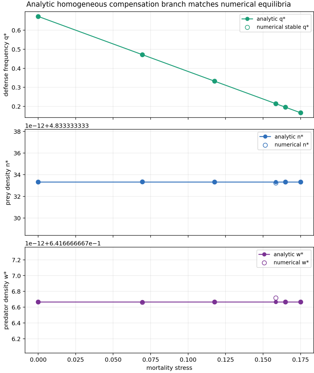
Figure 1: Analytic compensation branch for the linear trade-off parameterization, compared with numerical stable persistent equilibria. The plotted decline in q^*(s) shows the compensation mechanism: increasing mortality stress is balanced by lower prey defense, while n^* and w^* remain approximately fixed. The allowed conclusion is branch agreement and compensation in the tested parameterization, not global stability.
