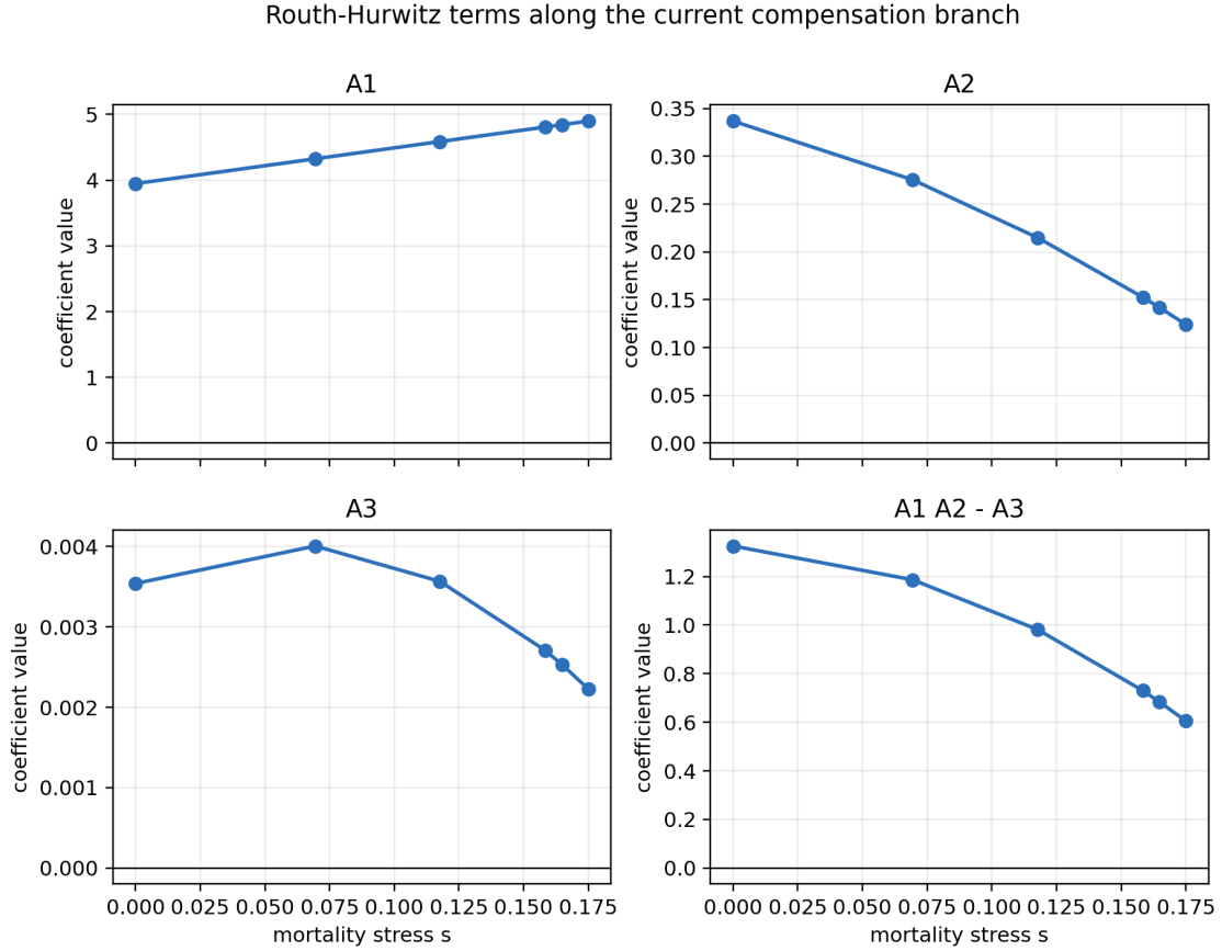
Figure 3: Routh–Hurwitz coefficient terms along the compensation branch. The plotted quantities are A_1 , A_2 , A_3 , and A_1A_2 - A_3 . Their positivity supports local stability at the tested stresses, but does not establish global basin attraction.
