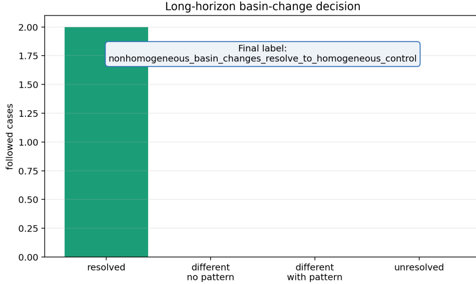
Figure 5: Long-horizon follow-up of the finite-amplitude non-homogeneous basin-changing cases. The figure summarizes whether basin-changing cases resolved to matched homogeneous controls, persisted as different basins, or retained spatial structure. The allowed conclusion is that the followed finite-horizon basin changes resolved without persistent spatial patterning.
