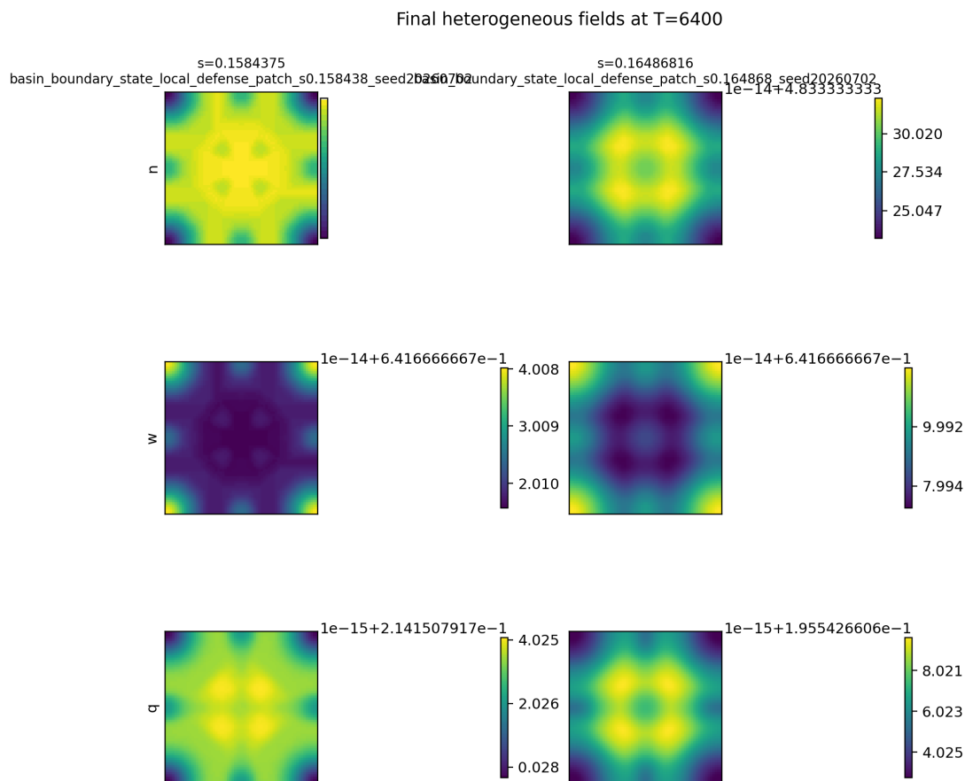
Figure 32: Final fields for the followed heterogeneous cases at the longest focused horizon.
