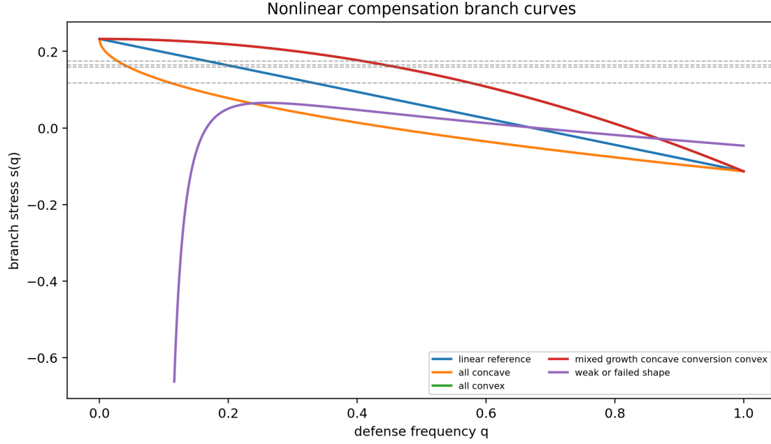
Figure 15: Generalized nonlinear compensation branch curves s(q) for selected endpoint-preserving trade-off shapes. Target stresses are marked for comparison.
