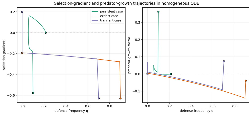
Figure 36: Representative ODE relationship between defense frequency q , the selection gradient on defense, and the predator growth factor.
