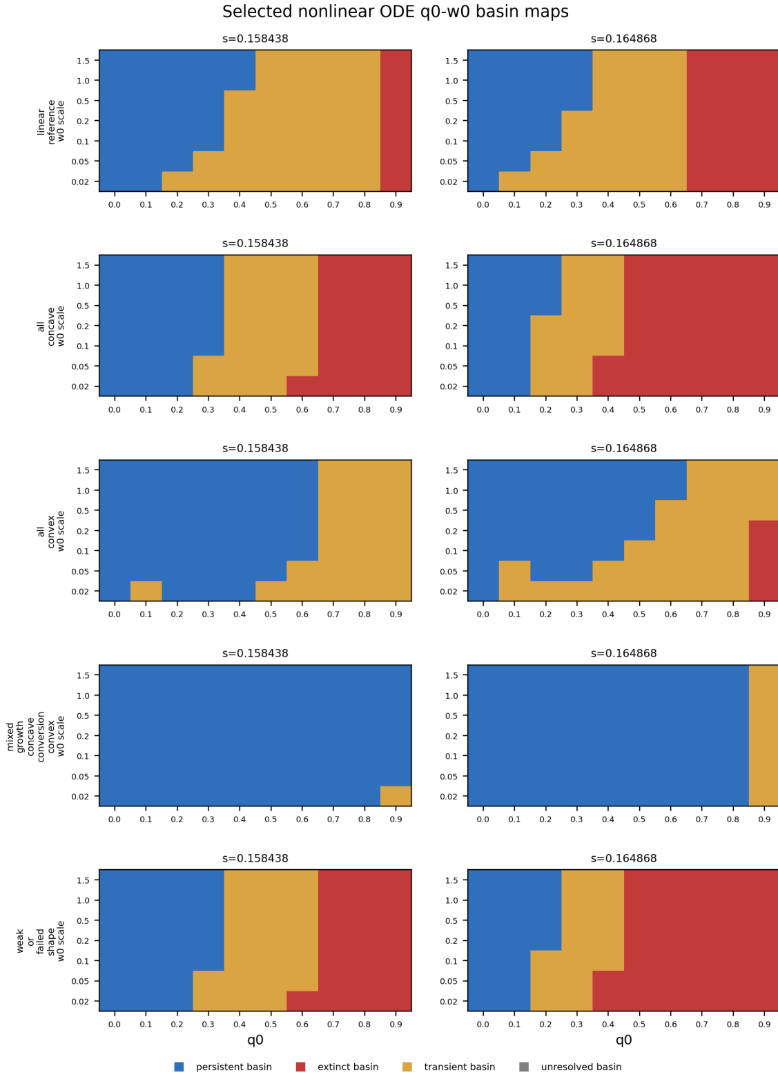
Figure 17: Selected homogeneous ODE basin maps for linear, concave, convex, mixed, and weak/failed nonlinear shape cases.
