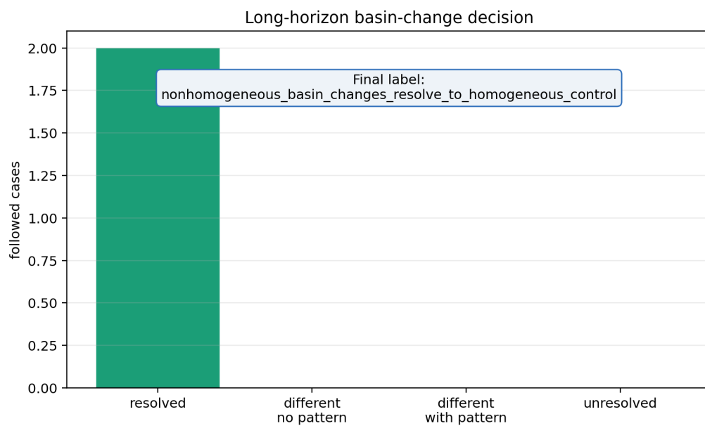
Figure 33: Decision summary for the long-horizon follow-up of the PR #23 basin-changing non-homogeneous cases.
