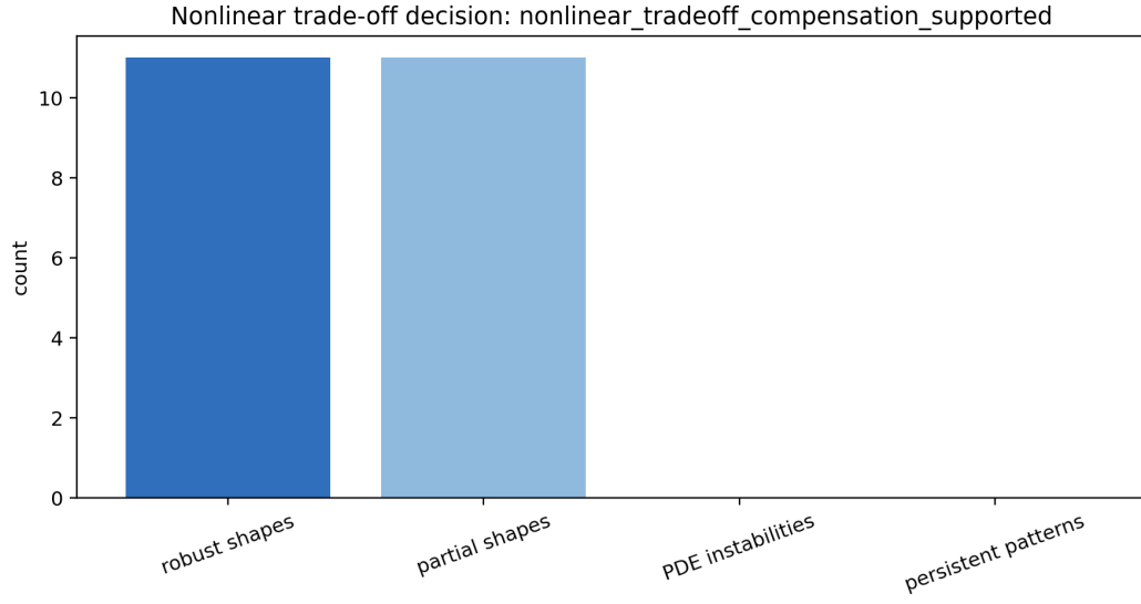
Figure 20: Final nonlinear trade-off extension decision summary. The supported label is conditional on the controlled shape grid and targeted PDE checks.
