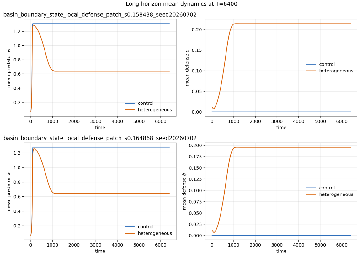
Figure 30: Long-horizon mean trajectories for the PR #23 basin-changing non-homogeneous cases and their matched homogeneous controls.
