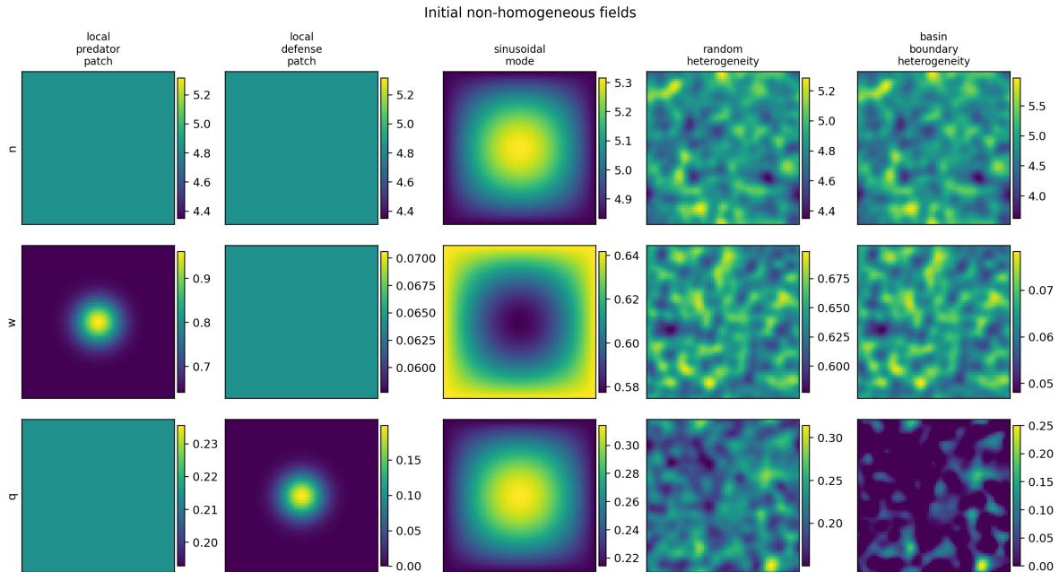
Figure 25: Representative non-homogeneous initial conditions used in the targeted nonlinear PDE perturbation tests.
