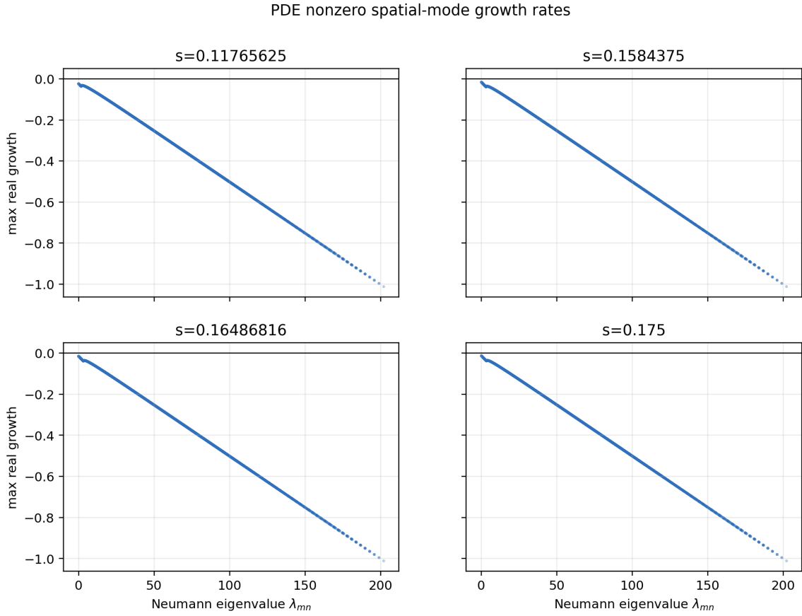
Figure 21: Nonzero Neumann spatial-mode growth rates along the homogeneous compensation branch under the current diffusion coefficients.
