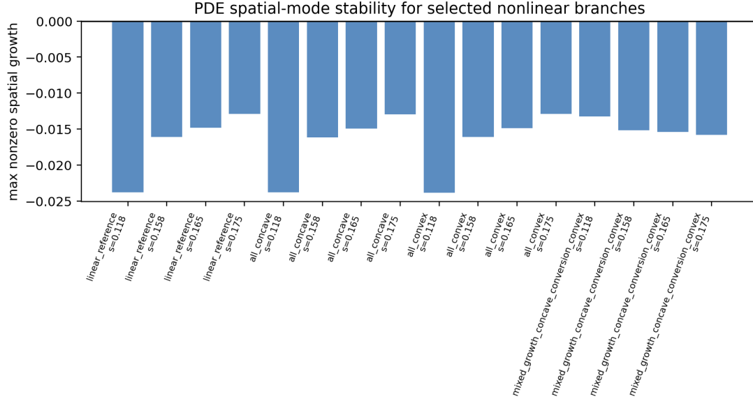
Figure 18: Maximum nonzero Neumann spatial-mode growth for selected nonlinear branch states. No selected stable branch case showed positive nonzero spatial growth.
