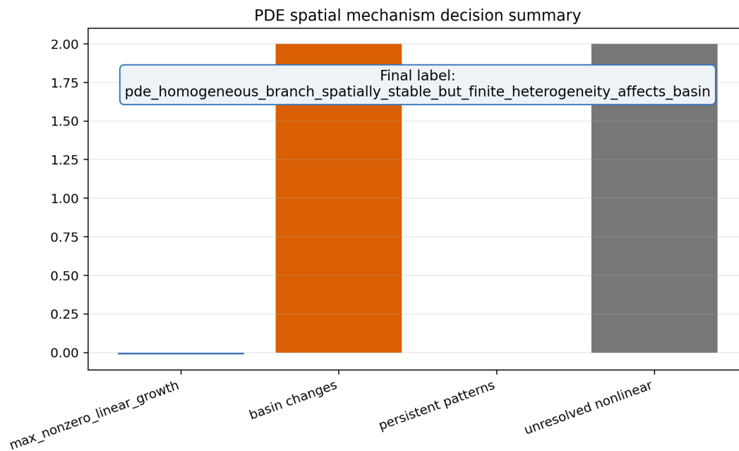
Figure 29: Decision summary for the PDE spatial-mode and finite-amplitude non-homogeneous perturbation analysis.
