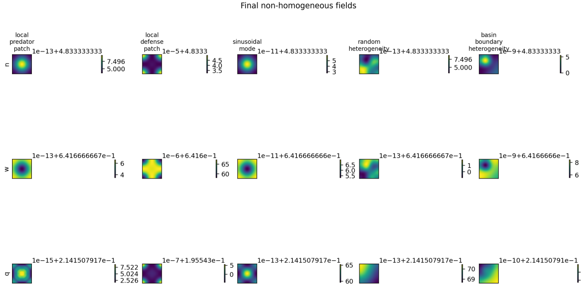
Figure 26: Final fields from representative non-homogeneous perturbation tests. Spatial variation decays in the representative saved fields.
