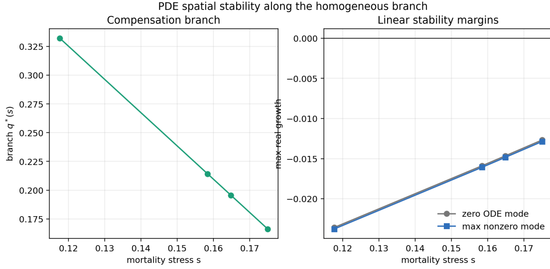
Figure 22: Spatial stability summary along the compensation branch. The largest nonzero mode growth rate remains negative at the tested stresses.
