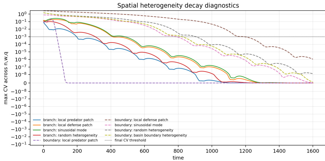
Figure 28: Spatial coefficient-of-variation diagnostics for selected non-homogeneous PDE perturbation tests.
