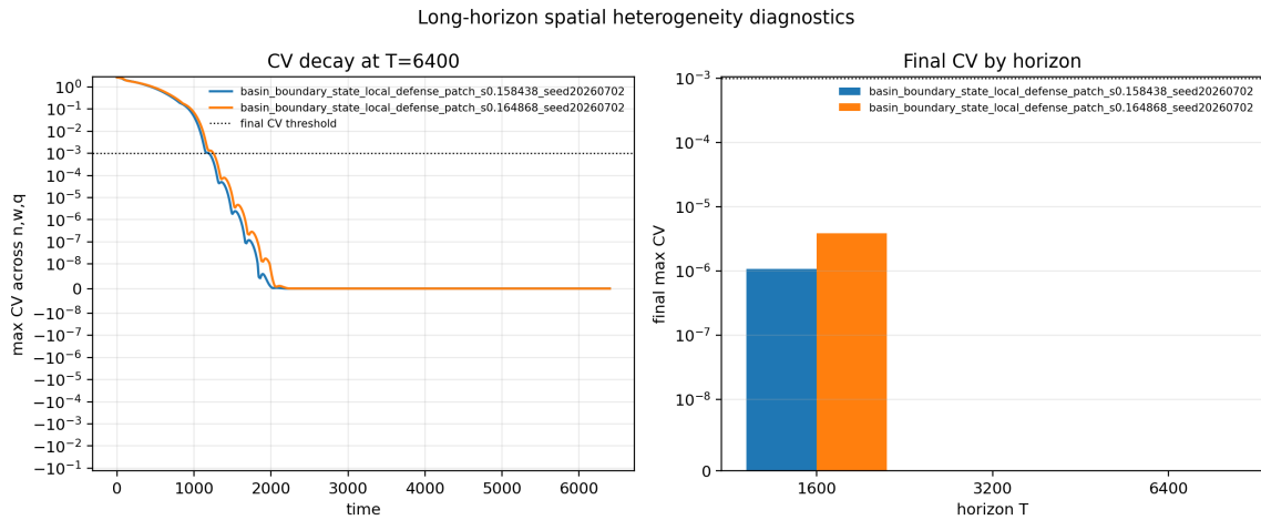
Figure 31: Spatial CV diagnostics for the long-horizon follow-up. Final spatial variation decays below the pattern-persistence threshold.
