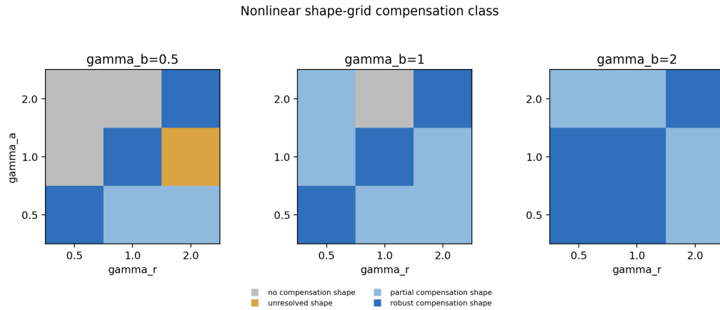
Figure 16: Controlled nonlinear shape-grid classification across \gamma_r, \gamma_a, \gamma_b \in \{0.5, 1, 2\} . The grid is structured and local, not a broad nonlinear trade-off scan.
