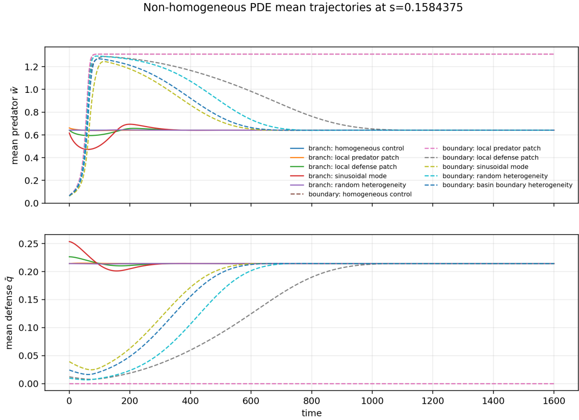
Figure 27: Spatial mean trajectories for homogeneous controls and selected non-homogeneous PDE perturbation tests.
