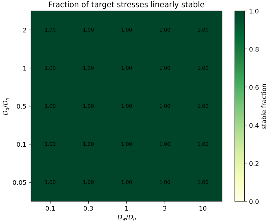
Figure 23: Controlled diffusion-ratio linear stability grid. The grid varies diffusion ratios only for the linear mode analysis and is not a nonlinear PDE parameter scan.
