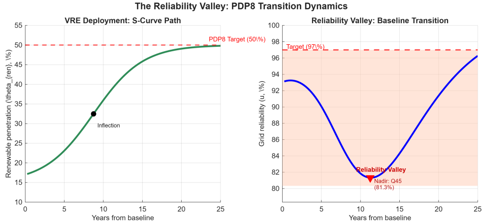
Figure 5: The Reliability Valley: PDP8 Transition Path
