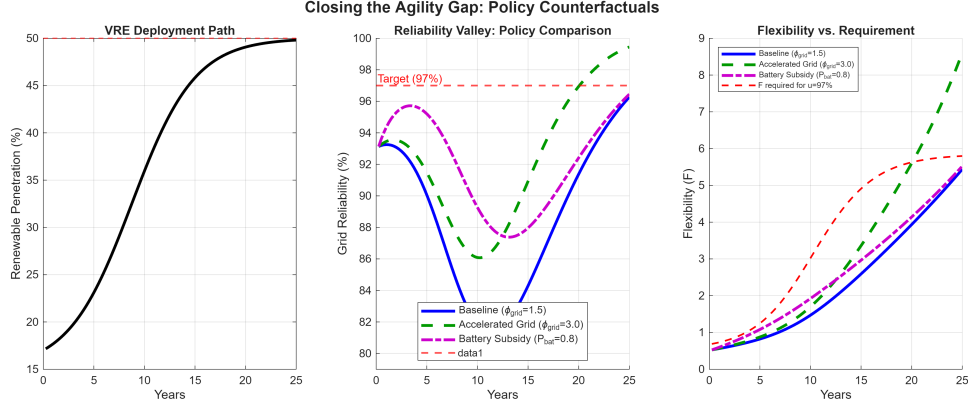
Figure 6: Closing the Agility Gap: Policy Counterfactuals. Left: shared S-curve renewable deployment path. Center: reliability paths under three scenarios—the battery subsidy (dash-dot) reduces the valley depth by 38.6%, while accelerated grid planning (dashed) shortens the valley duration by 20%. Right: flexibility accumulation versus the level required for 97% reliability.
