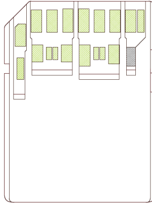
Figure H – 3: Standard SD Express G4L1 (Gen 4 1 lane) Card simplified view of pads side
