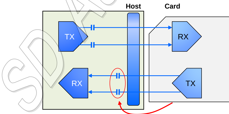
Figure 8-1 : Placement of AC coupling capacitors
