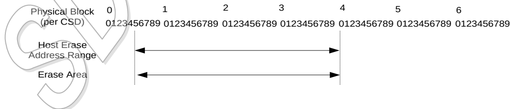
Figure 5-2 : ERASE_BLK_EN = 1 Example
