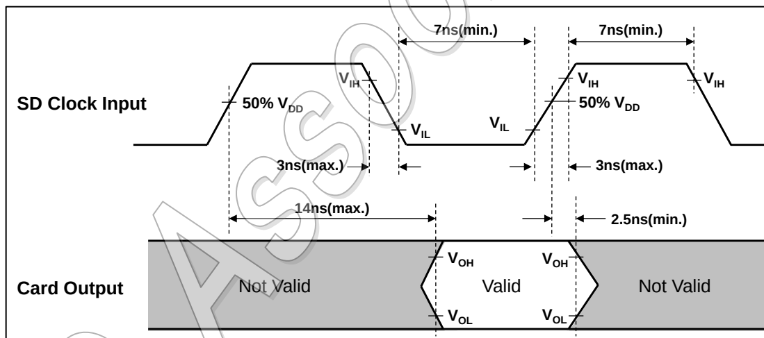
Figure 6-13 : Card Output Timing (High Speed Mode)
