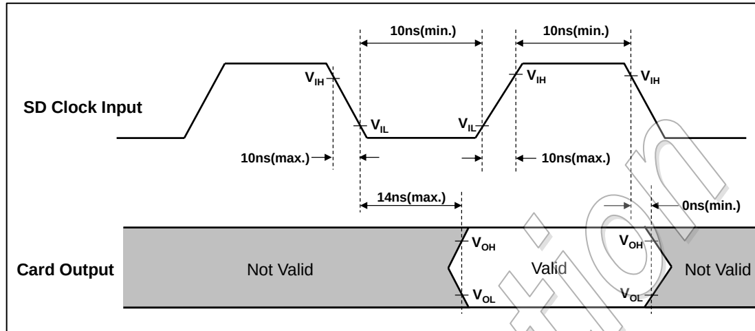
Figure 6-11 : Card Output Timing (Default Speed Mode)
