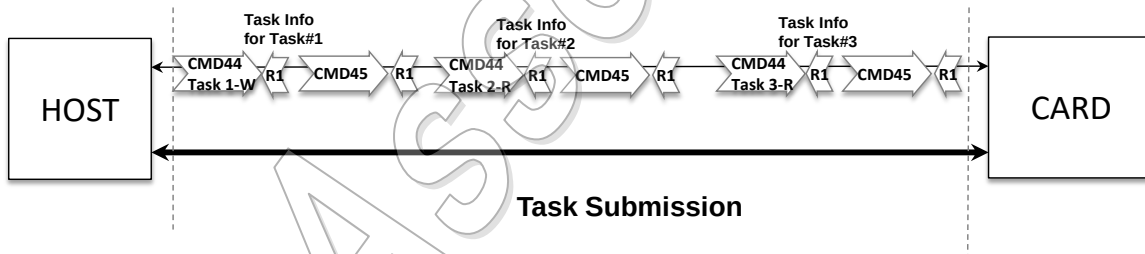
Figure 4-71 : Illustration of Task Submission
