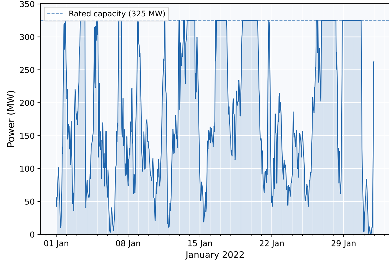
Thesis Wind Farm Power Output
