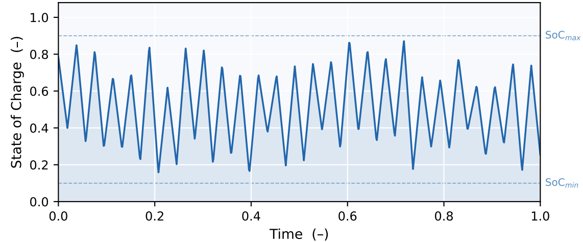
Battery Dispatch (SoC)
