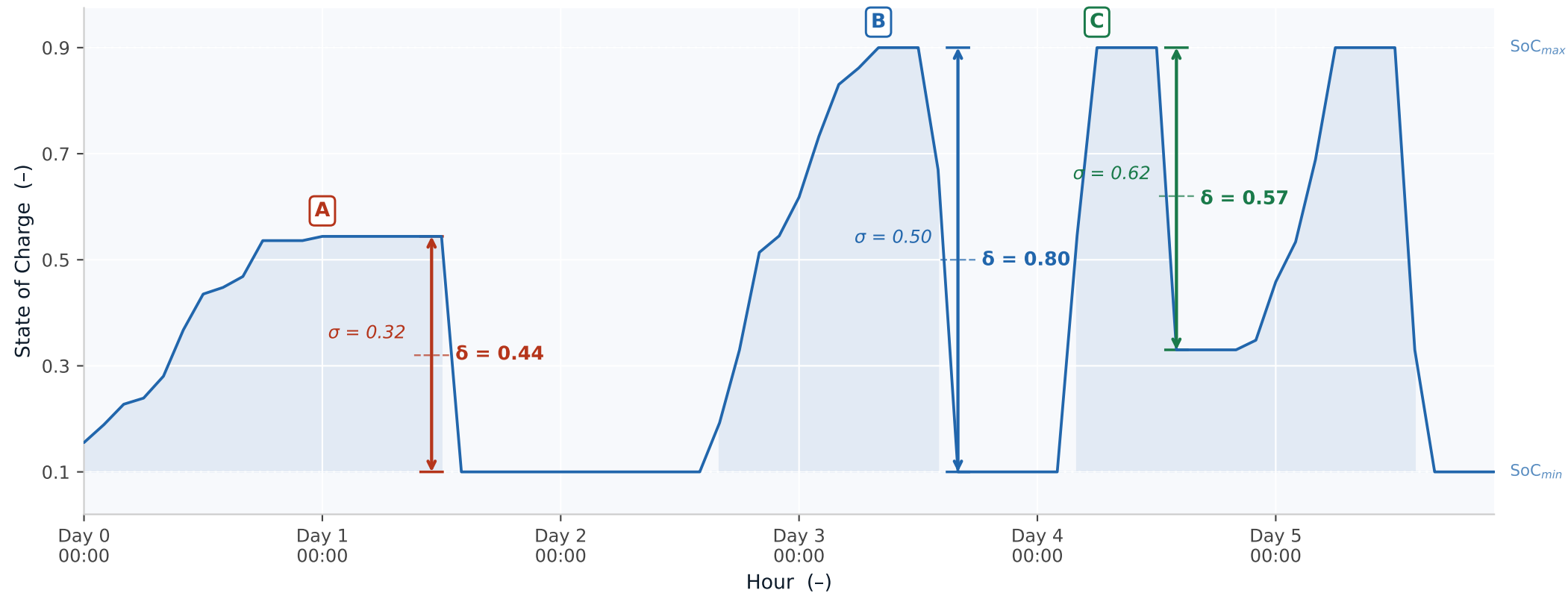
SoC Rainflow Cycles for a Representative Week (August 2022, IEA Task Force 50 site)
