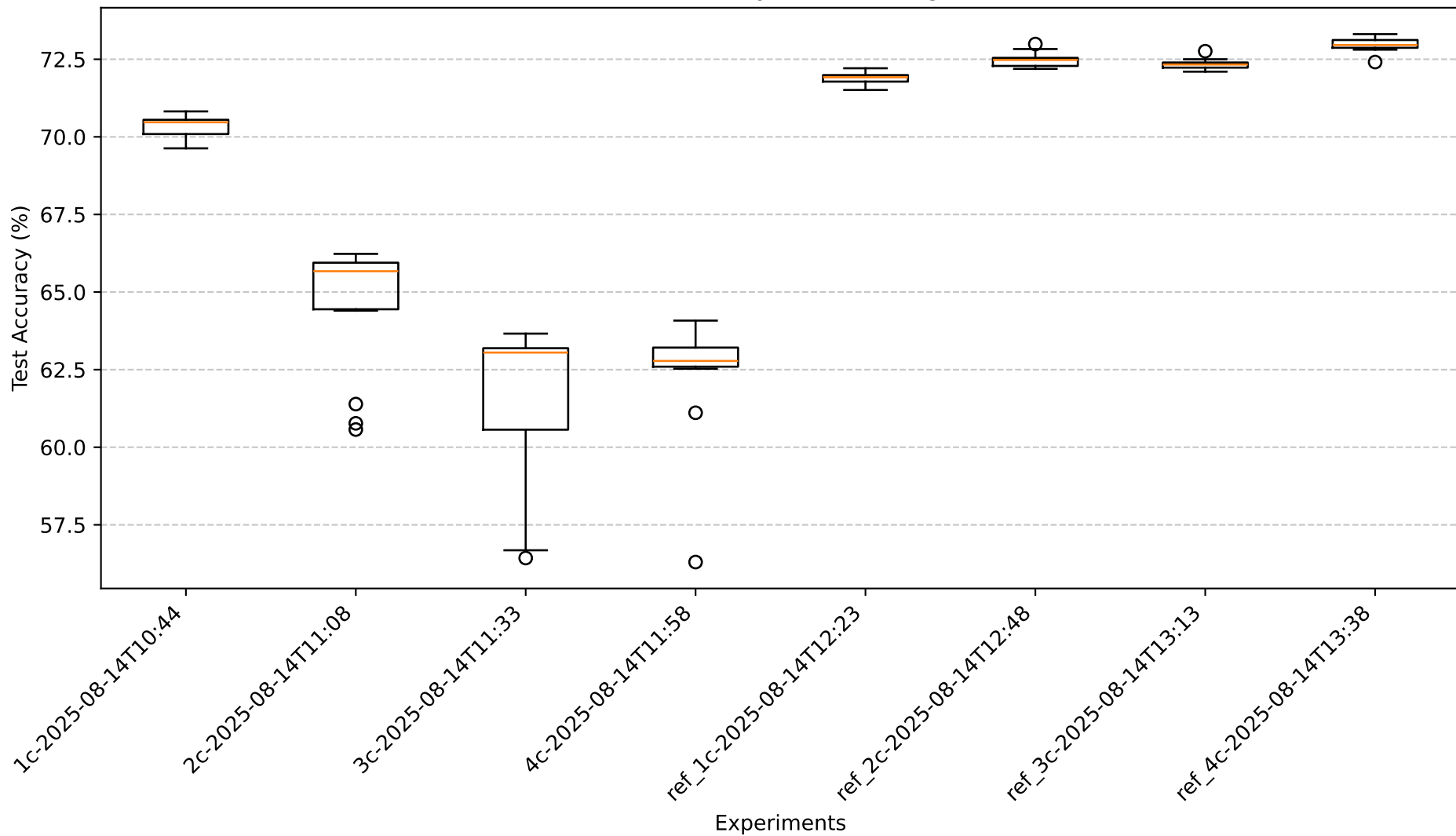
Final Test Accuracy of Defending Nodes
