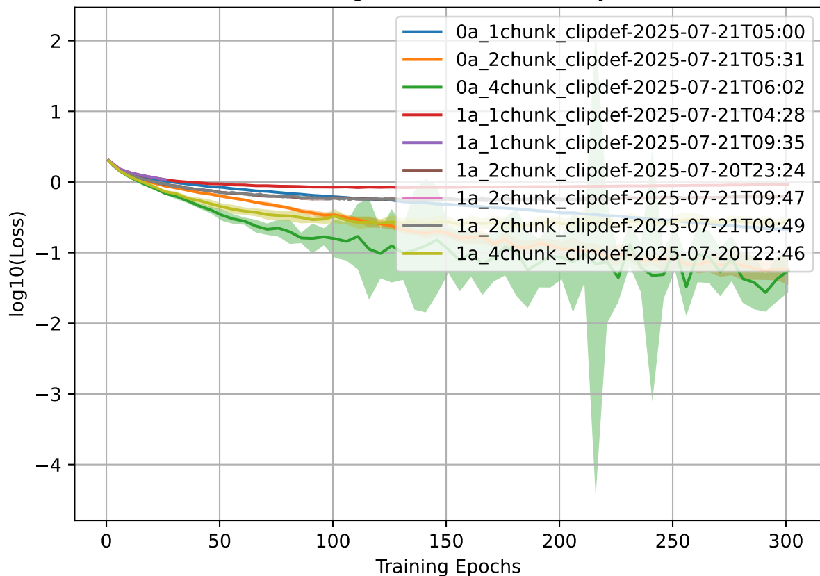
Training Loss (Defenders Only)
