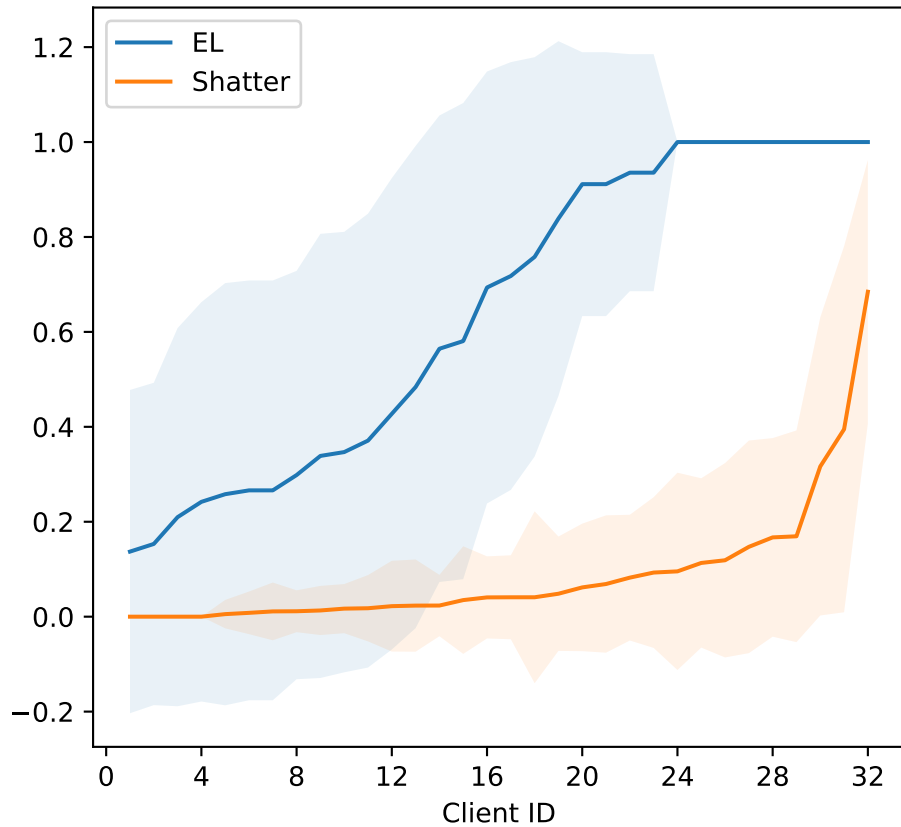
Linkability Attack per Client
