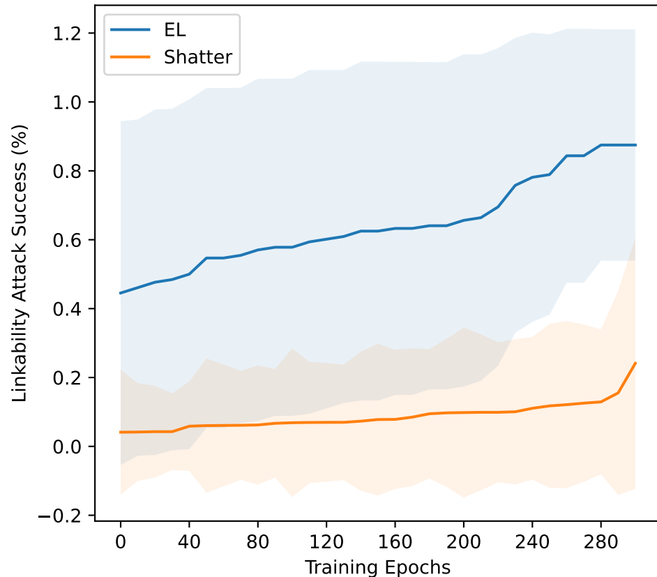
Linkability Attack per Iteration
