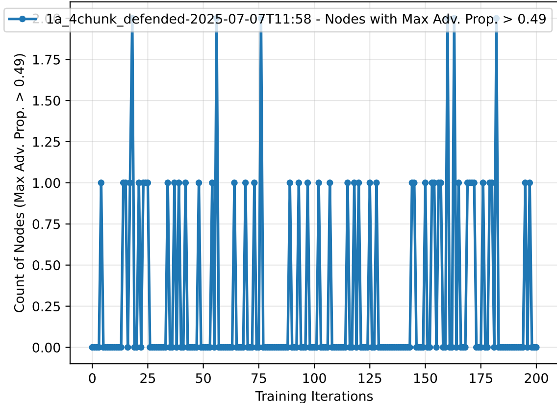
Count of Nodes with High Adversarial Influence Over Iterations
