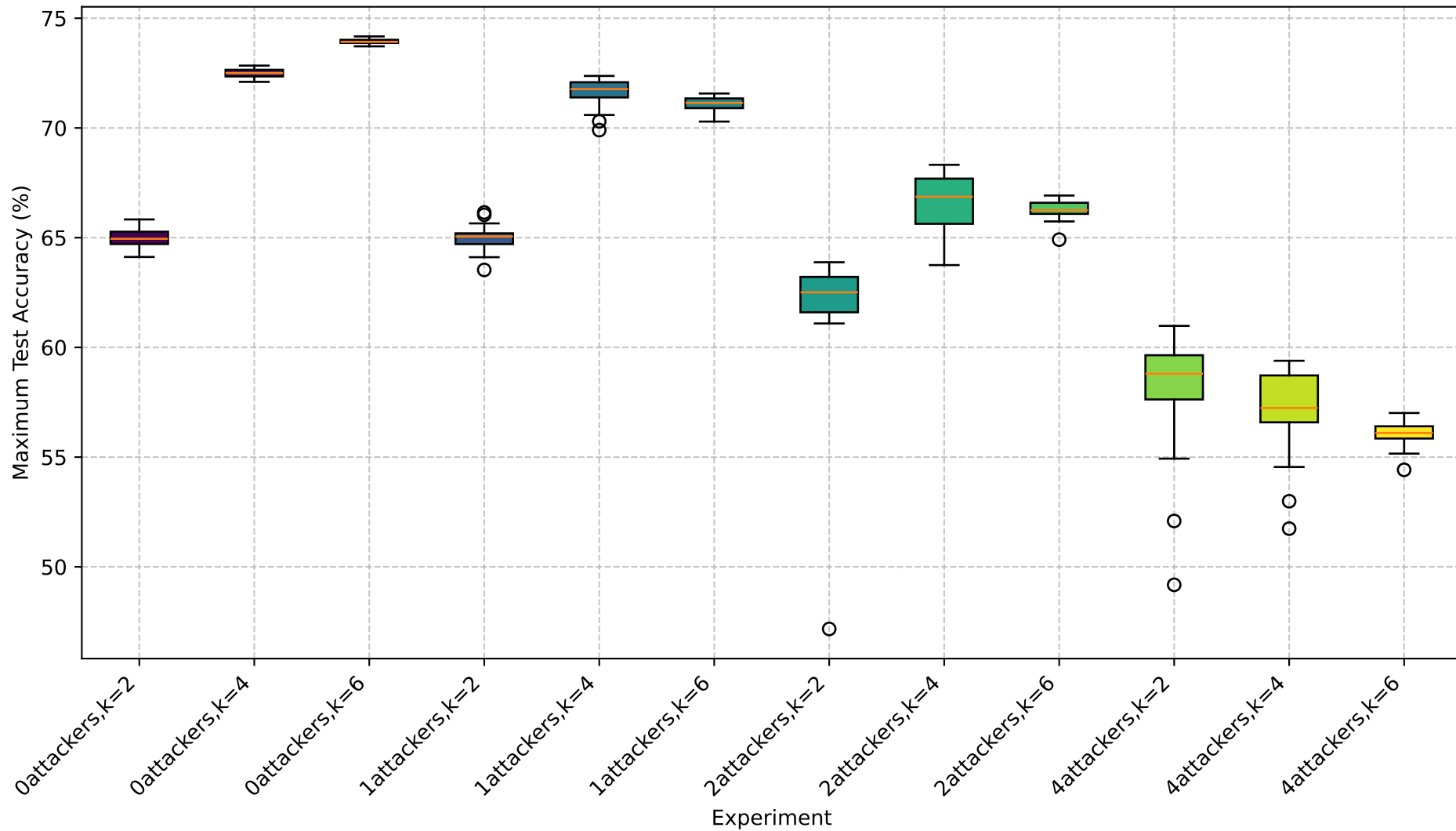
Maximum Test Accuracy Distribution by Experiment
