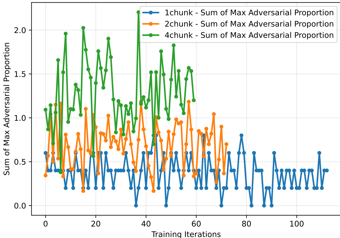
Sum of Max Adversarial Proportion Over Iterations
