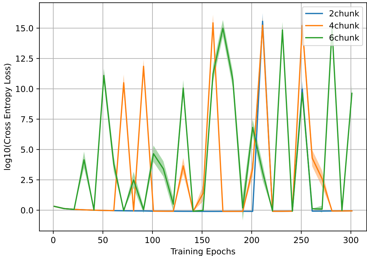
Convergence (Test Loss - Defenders Only)
