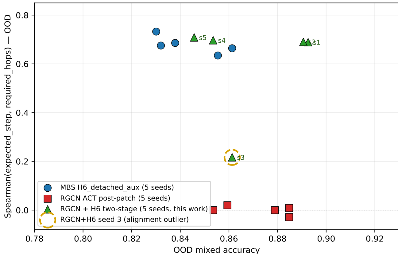
Accuracy vs halting policy alignment (5 seeds \times 3 configurations)
