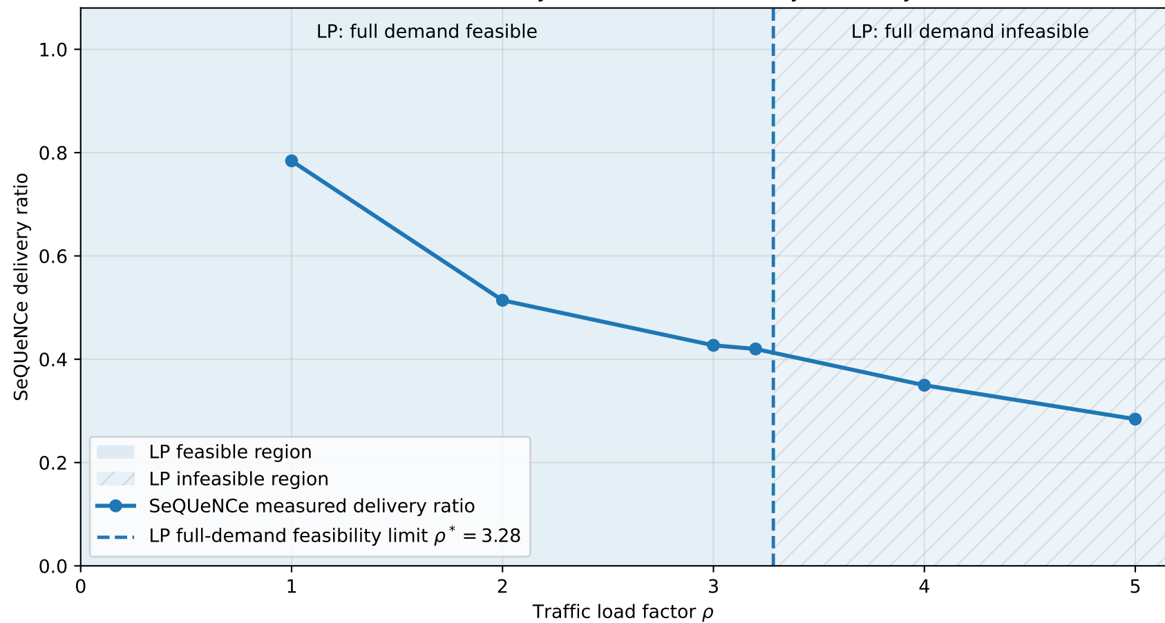
End-to-end delivery ratio and LP feasibility boundary
