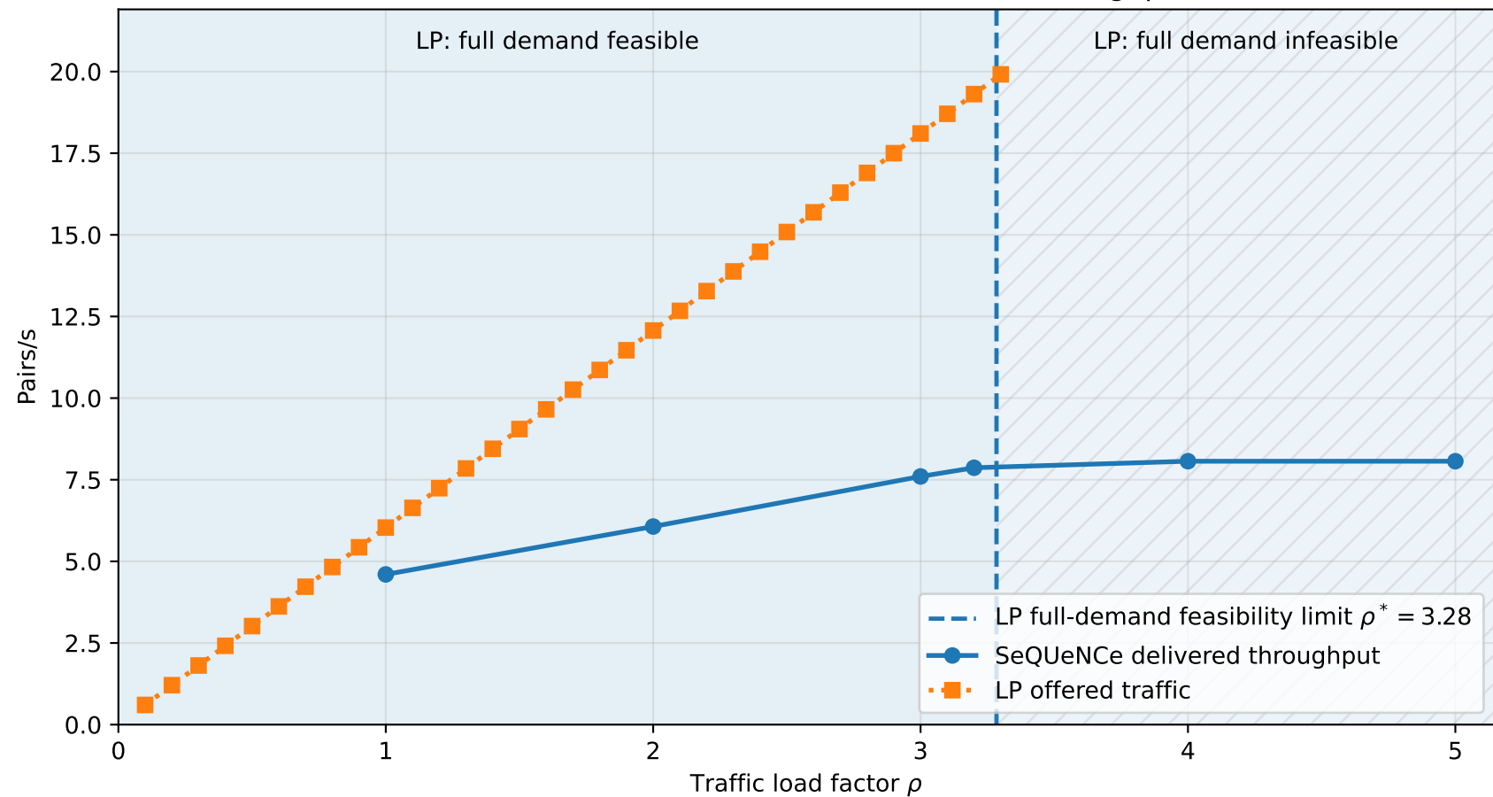
LP offered traffic and SeQUeNCe delivered throughput
