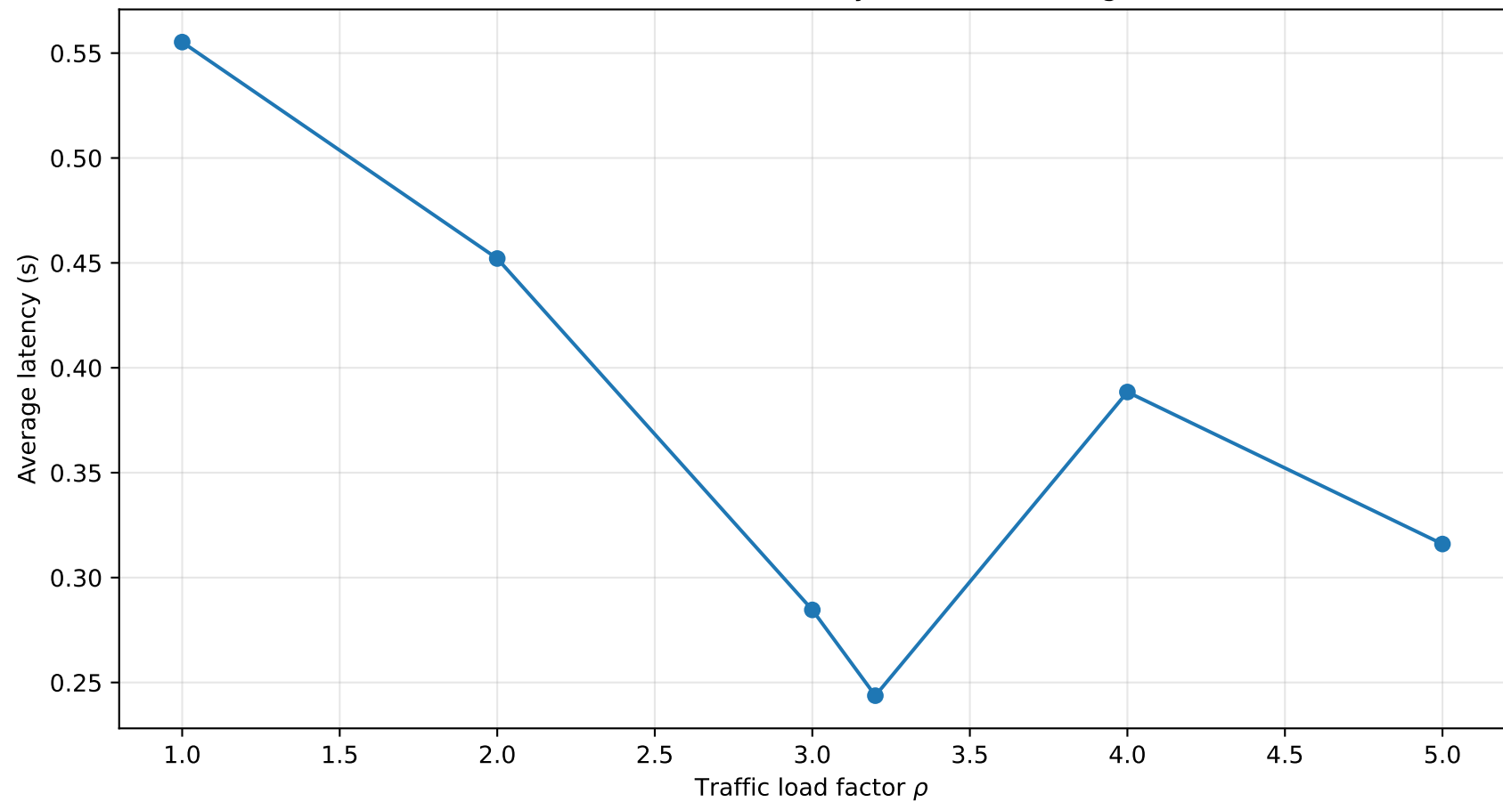
SeQUeNCe end-to-end latency under increasing load
