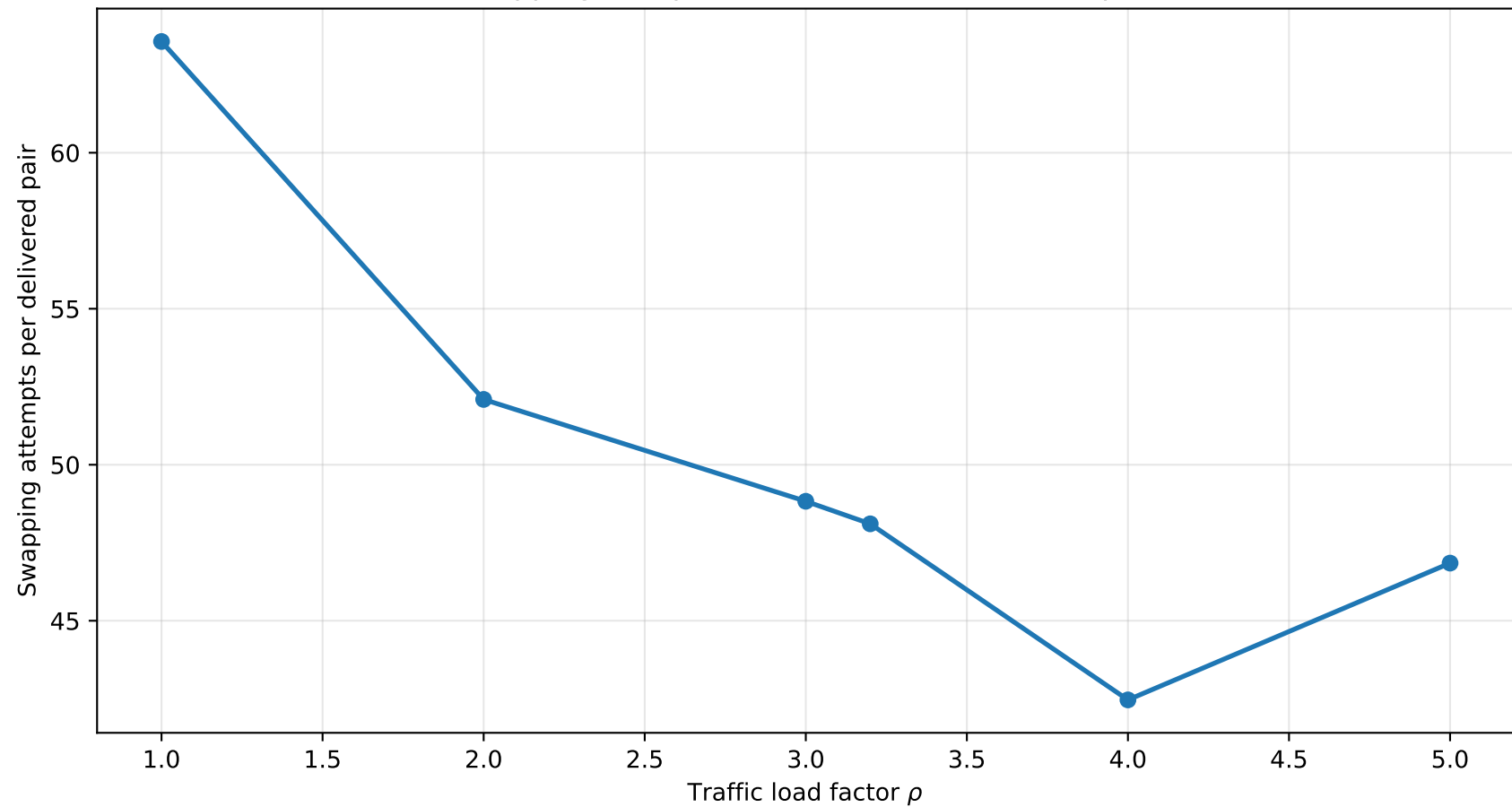
Swapping cost per delivered end-to-end Bell pair
