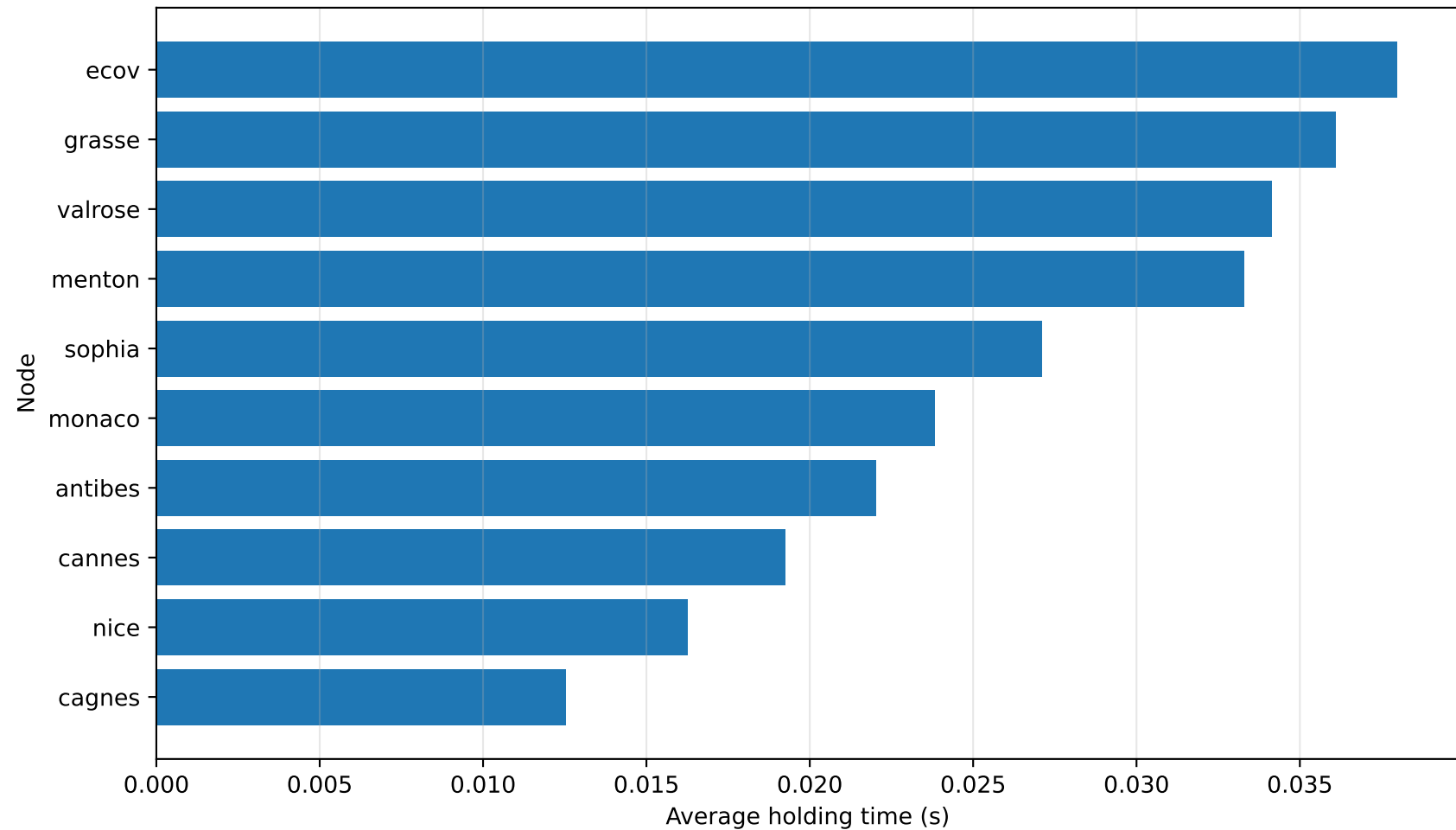
Average quantum-memory holding time at \rho = 3.20
