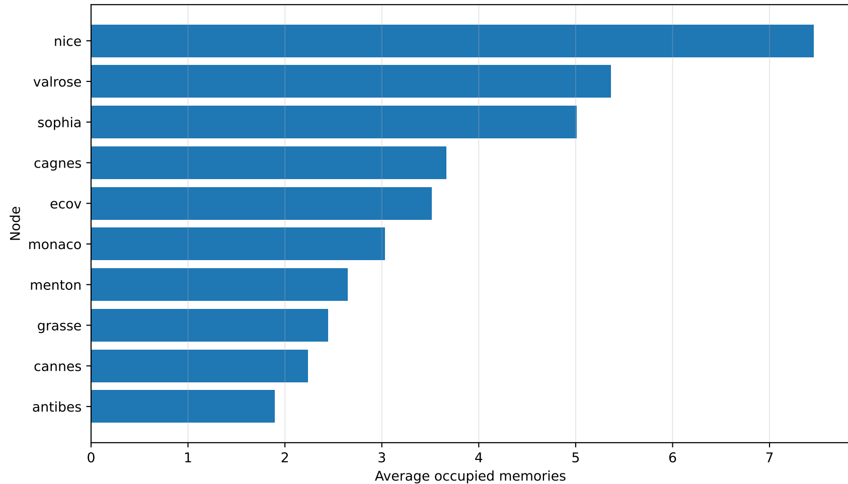
Average quantum-memory occupancy at \rho = 3.20
