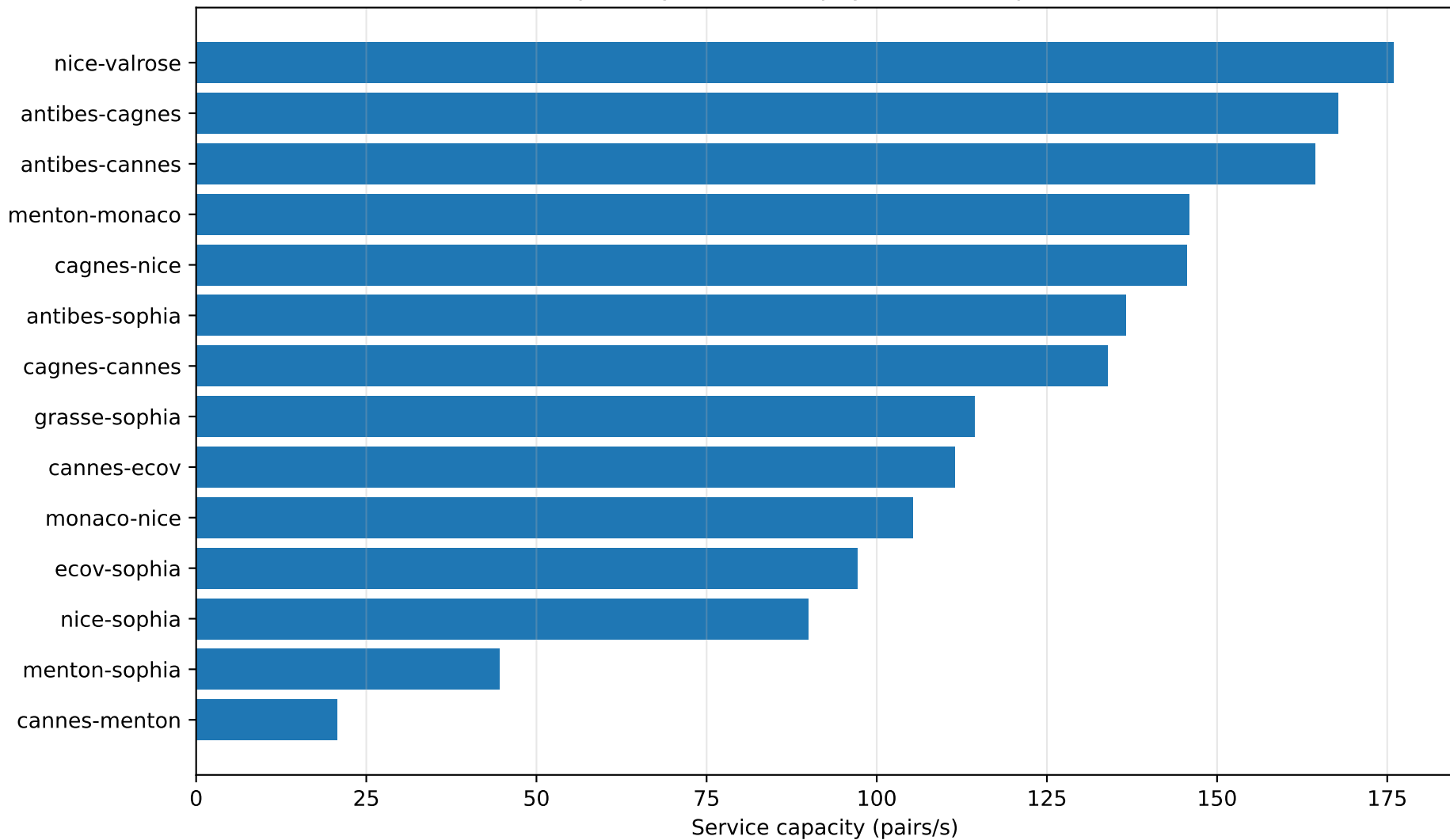
Empirically calibrated physical-link capacities
