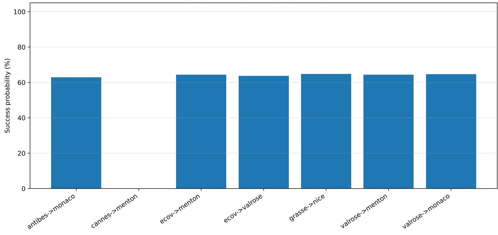
Swapping success probability by flow at \rho = 3.20
