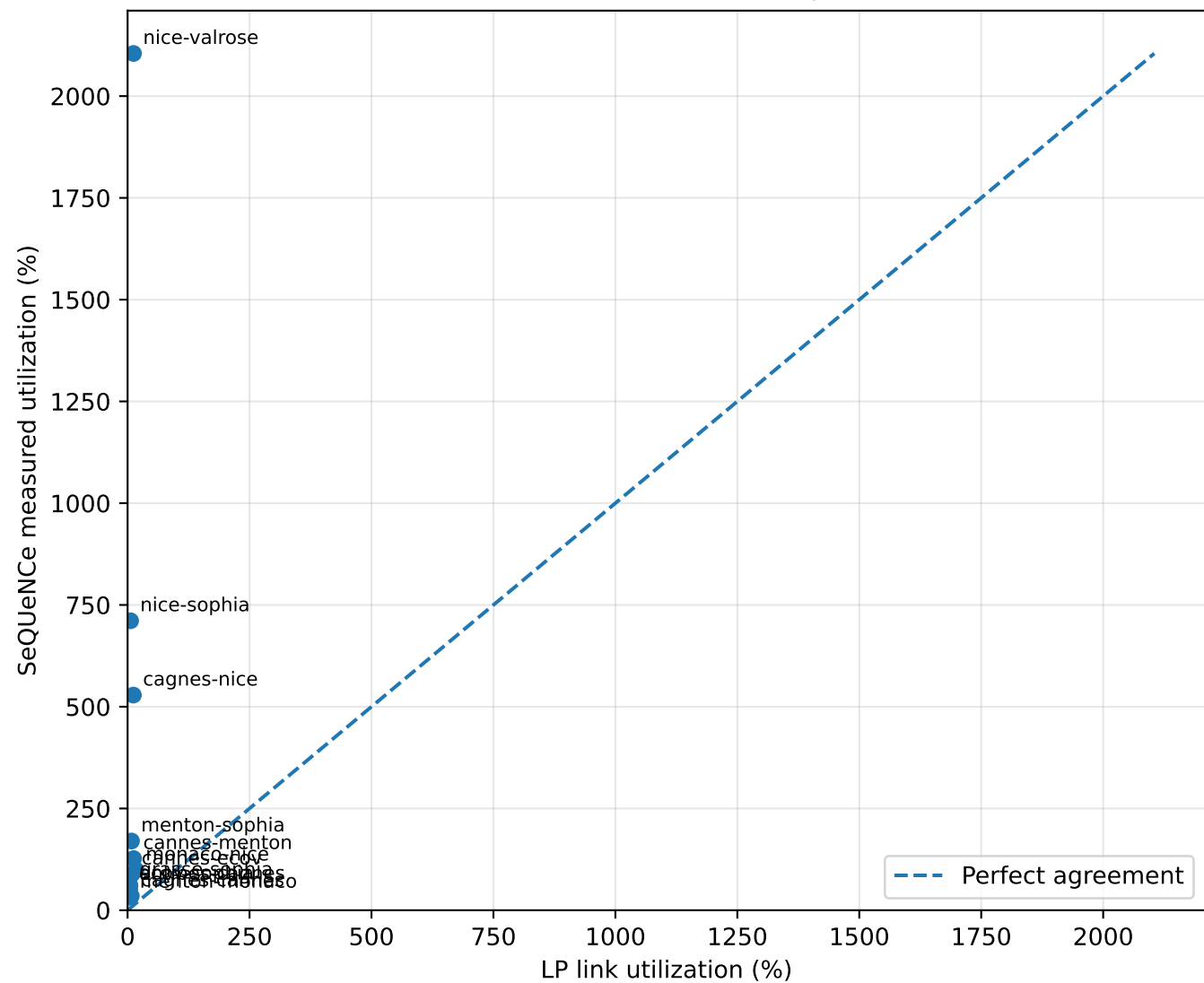
Link-utilization validation at \rho = 3.20
