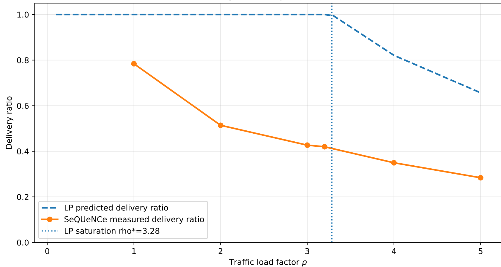
End-to-end delivery ratio: LP prediction vs SeQUeNCe
