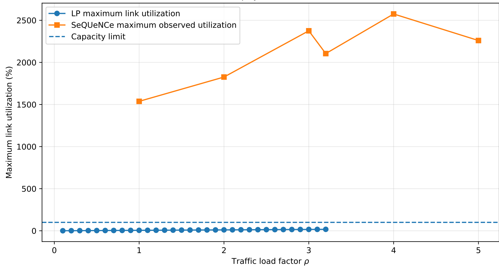
Maximum physical-link utilization
