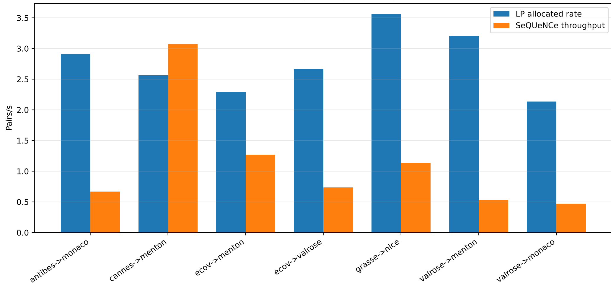
Flow-level throughput comparison at \rho = 3.20
