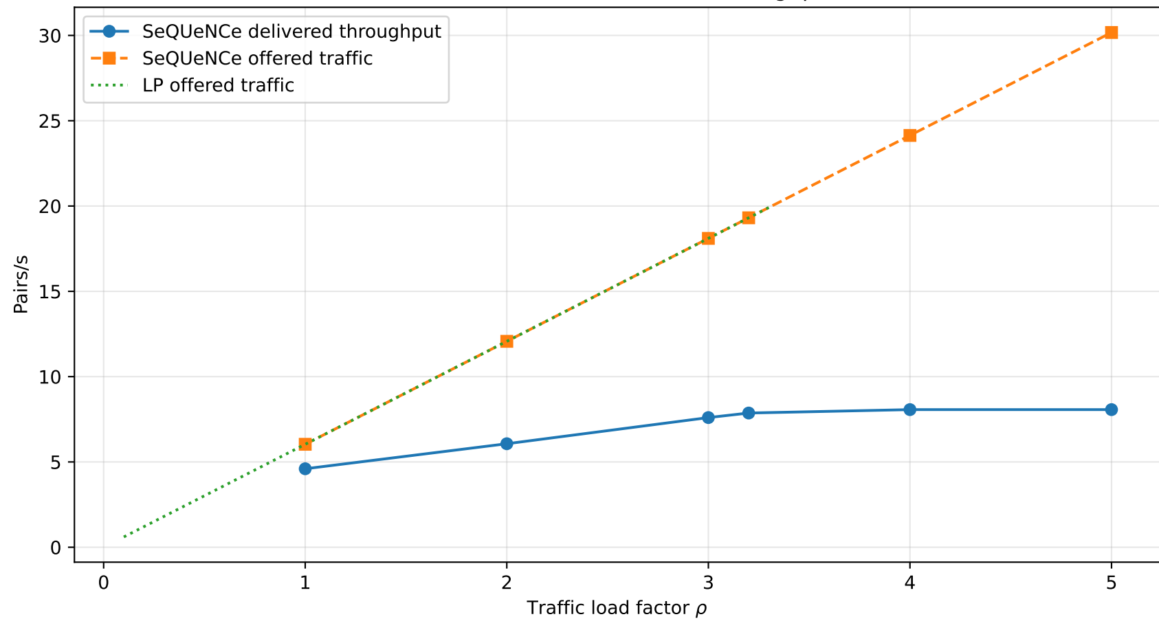
Offered traffic and delivered throughput
