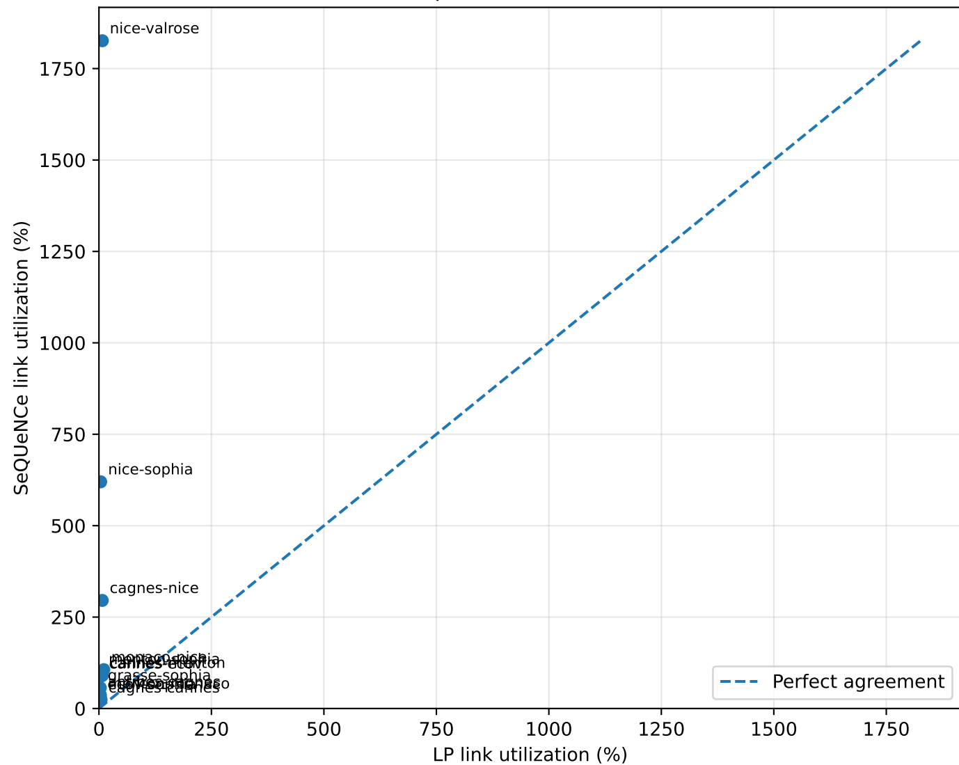
Link utilization: LP prediction vs SeQUeNCe ( \rho=2.00 )
