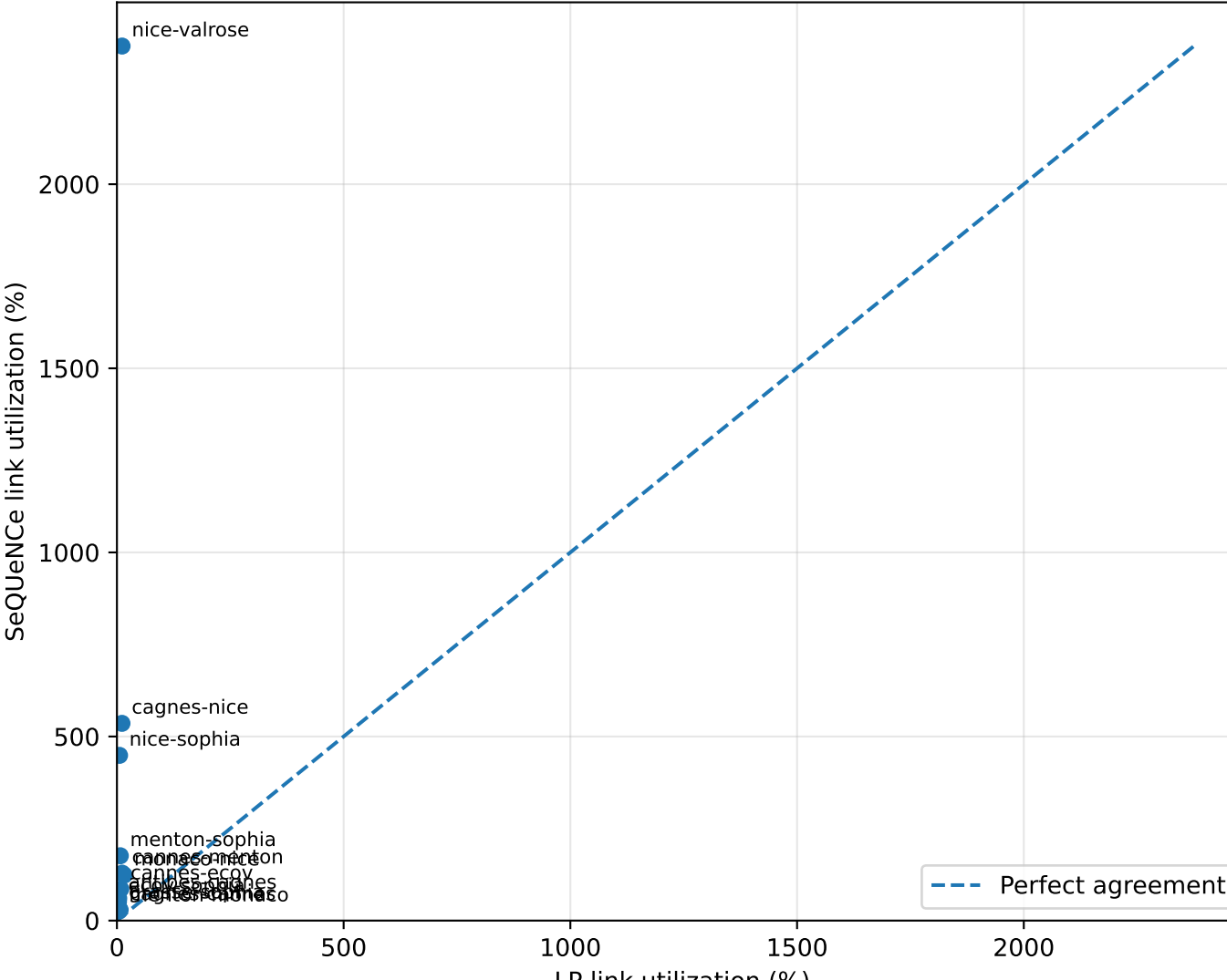
Link utilization: LP prediction vs SeQUeNCe ( \rho=3.00 )
