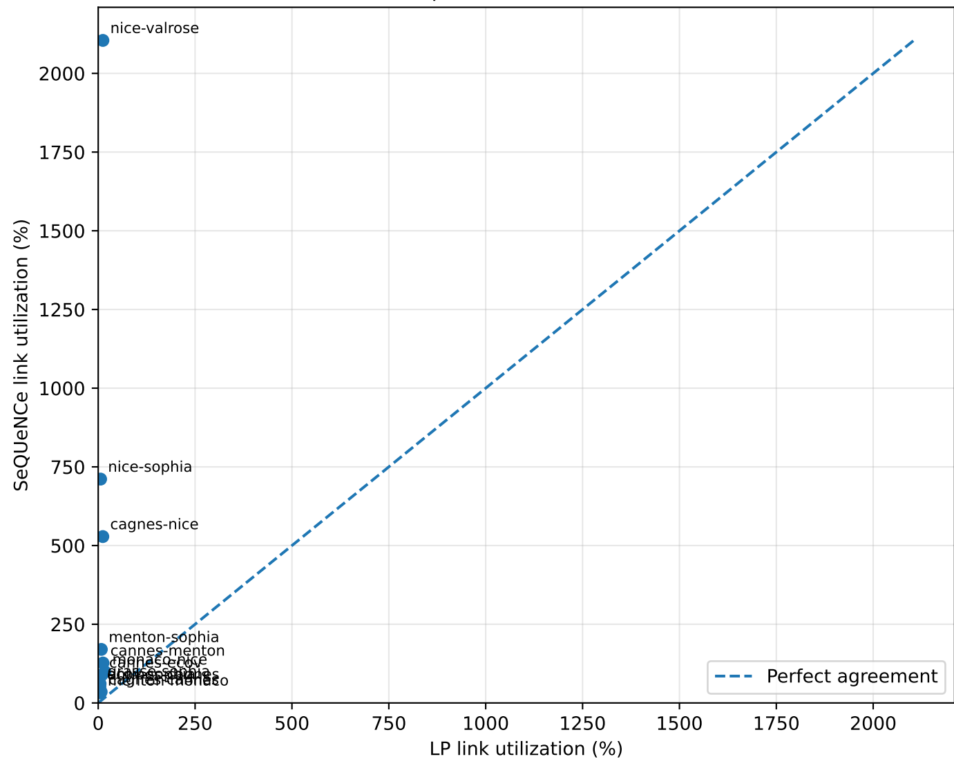
Link utilization: LP prediction vs SeQUeNCe (rho=3.20)
