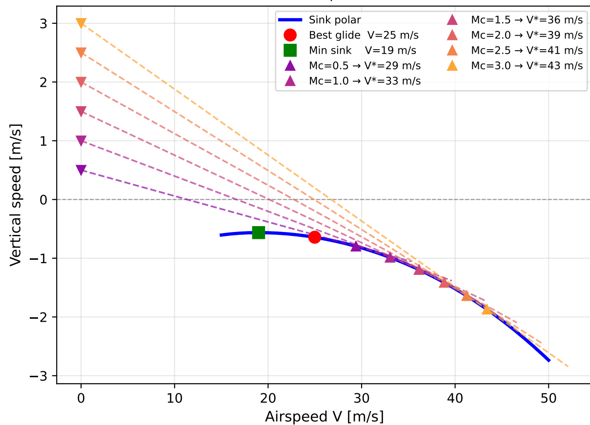
Glider polar
