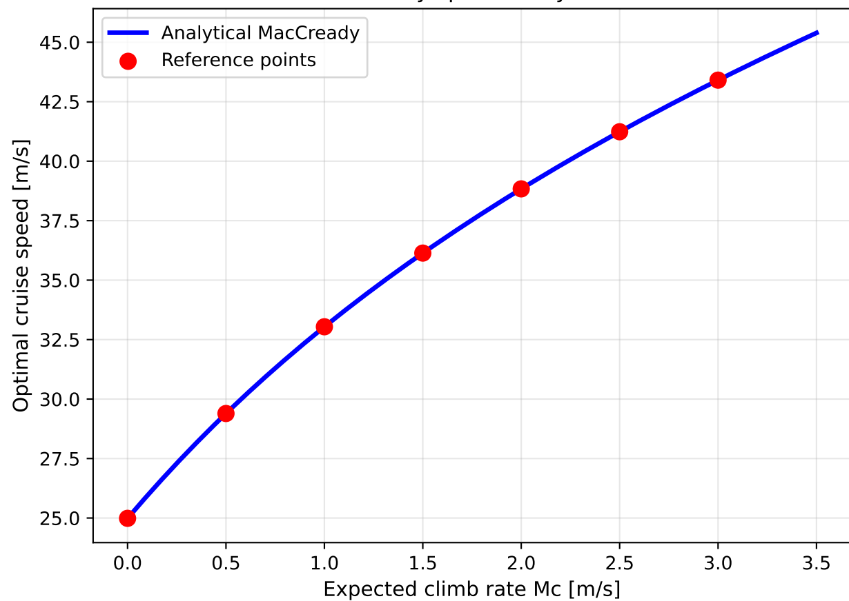
MacCready speed-to-fly curve
