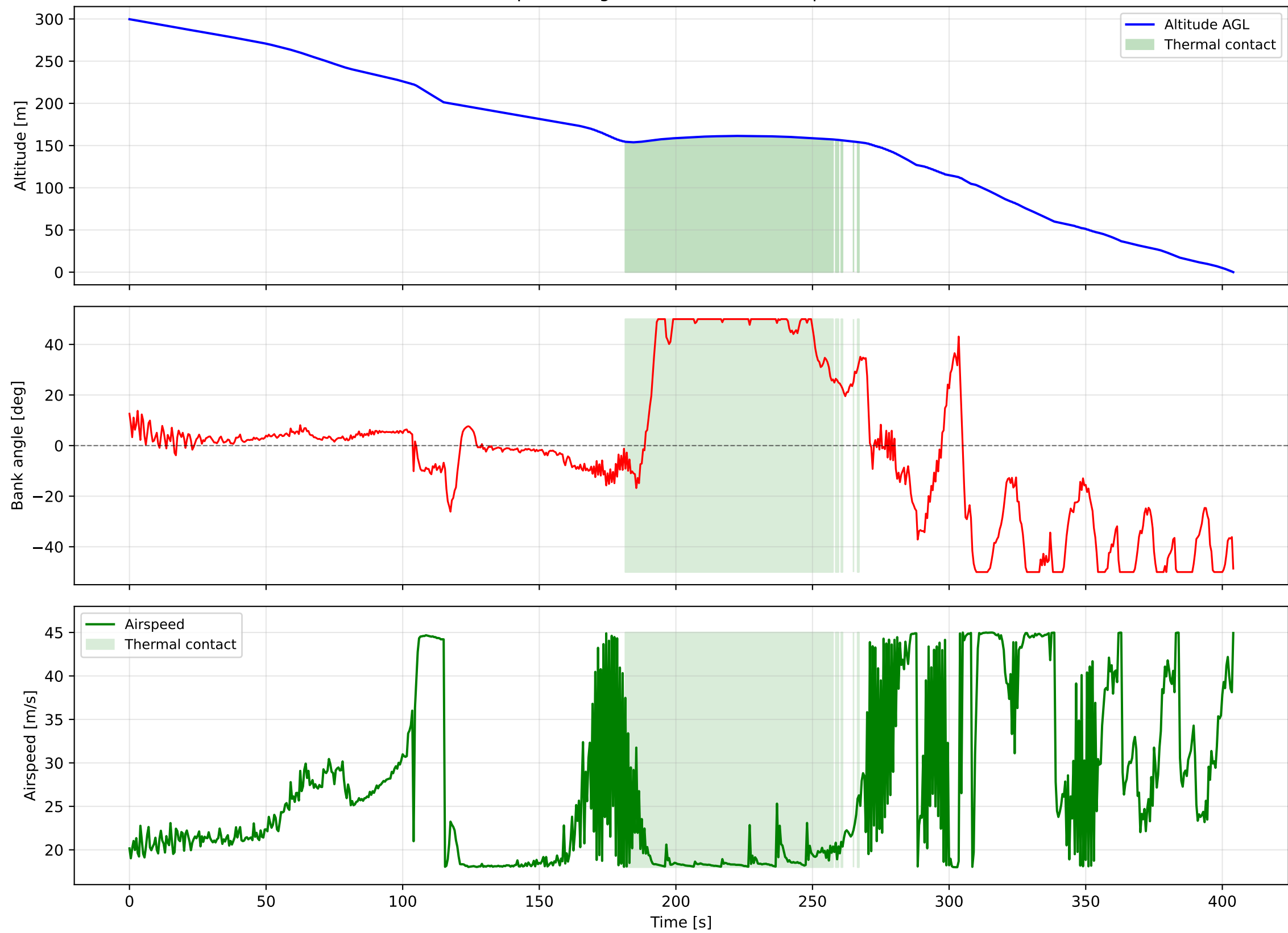
Episode flight: altitude, bank, airspeed
