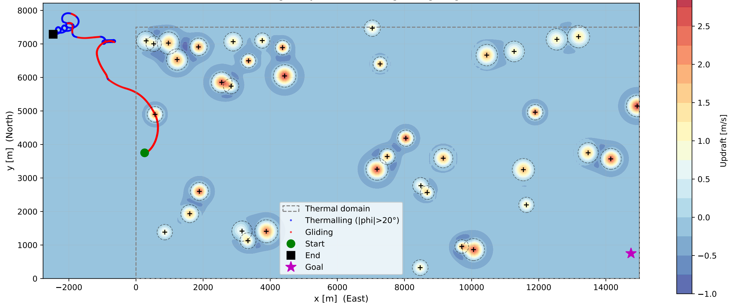
Climb-then-glide cycle: blue=circling, red=gliding
