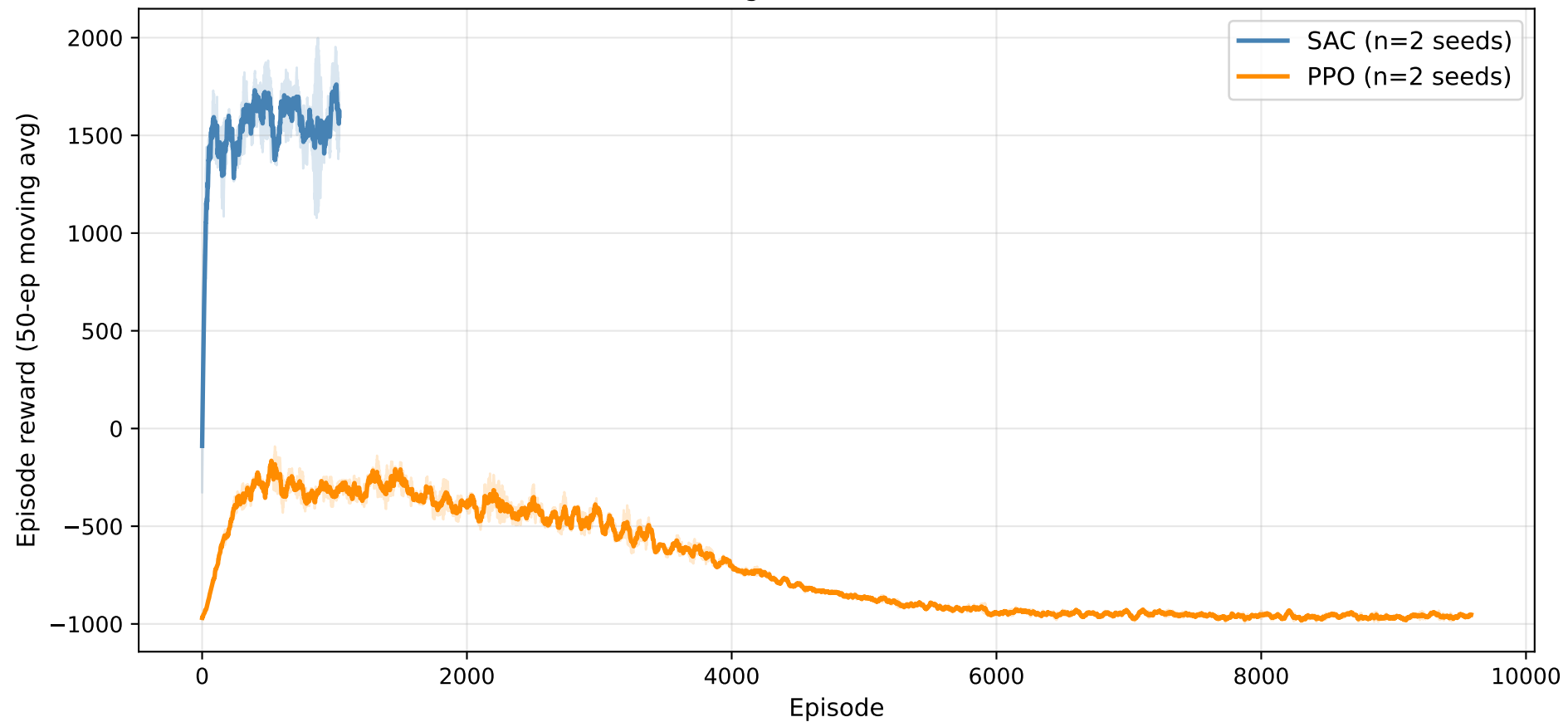
Learning curves: SAC vs PPO
