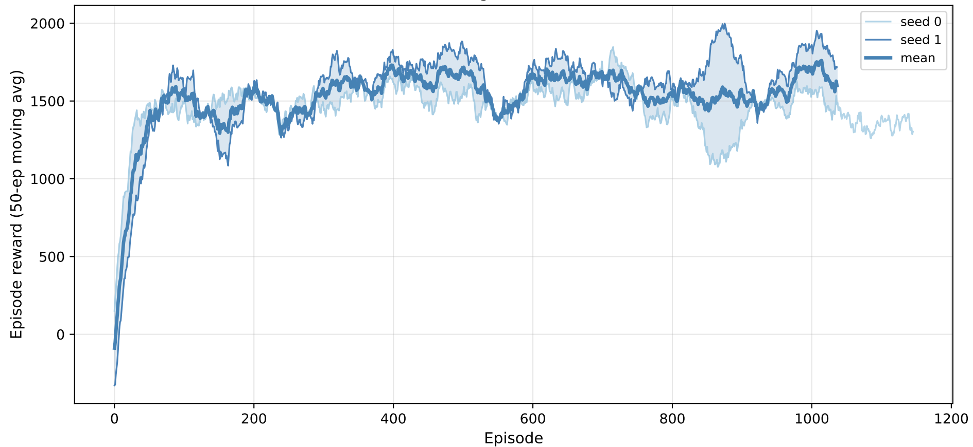
SAC learning curves (2 seed(s))
