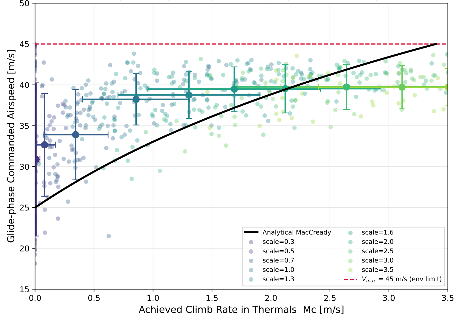
Learned Speed-to-Fly vs Analytical MacCready (SAC, 2 seed(s) pooled)
