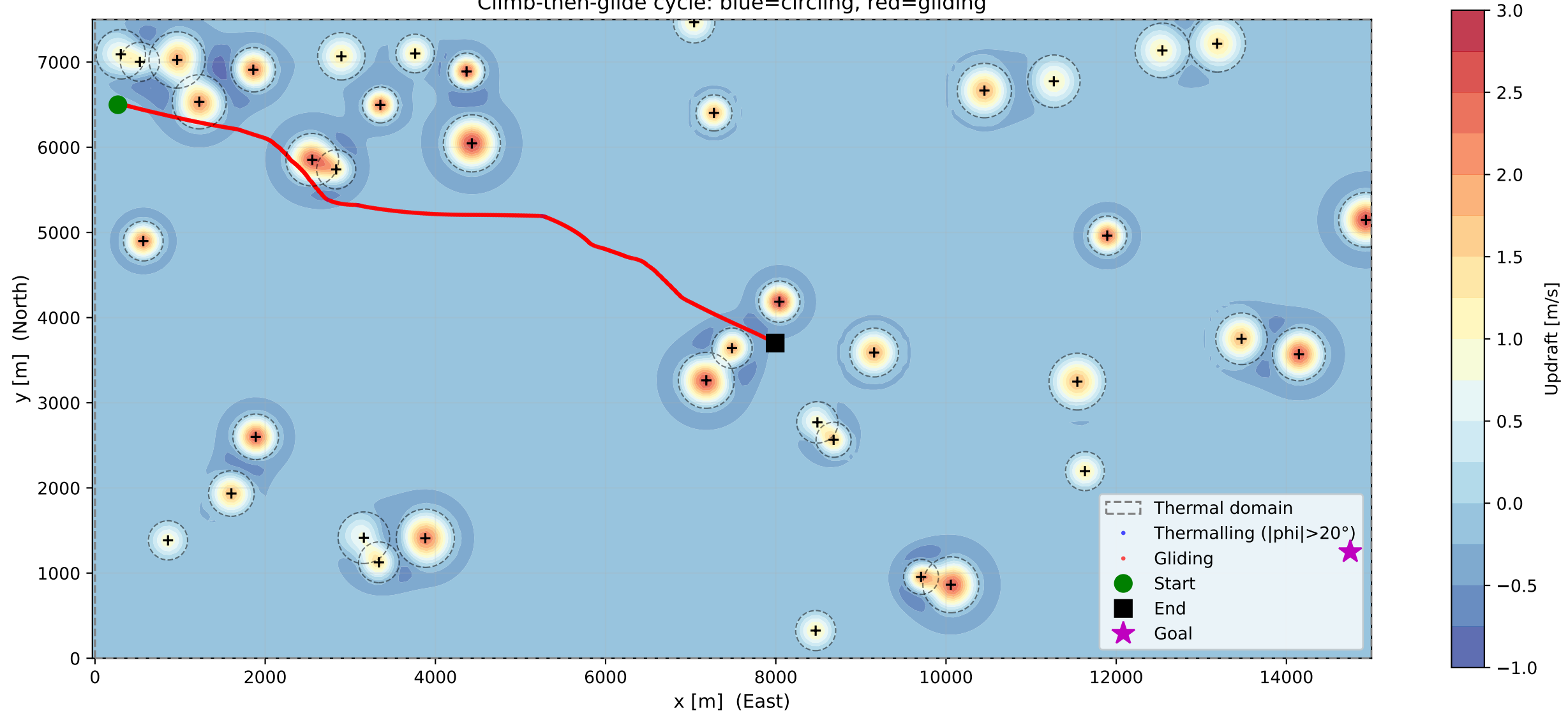
Climb-then-glide cycle: blue=circling, red=gliding
