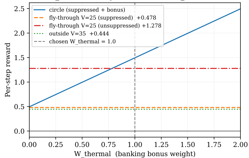
W_thermal sweep (w = 2.0 m/s, alt_scale = 1)
