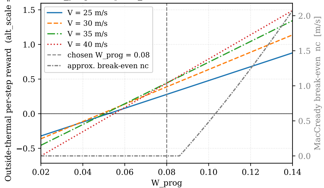
W_prog sweep ( W_{\text{alt}} = 1.0 , headwind = 5.0 m/s)
