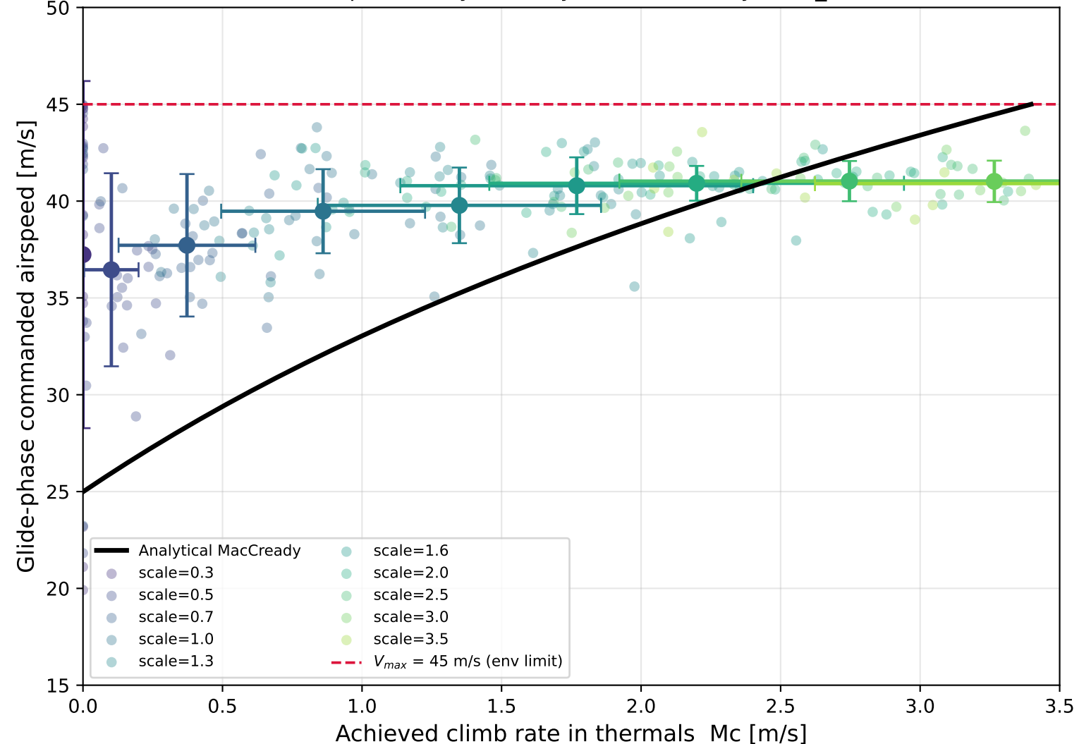
Learned speed-to-fly vs analytical MacCready (sac_seed0)
