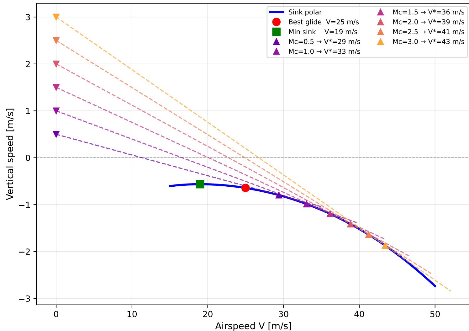
Glider polar
