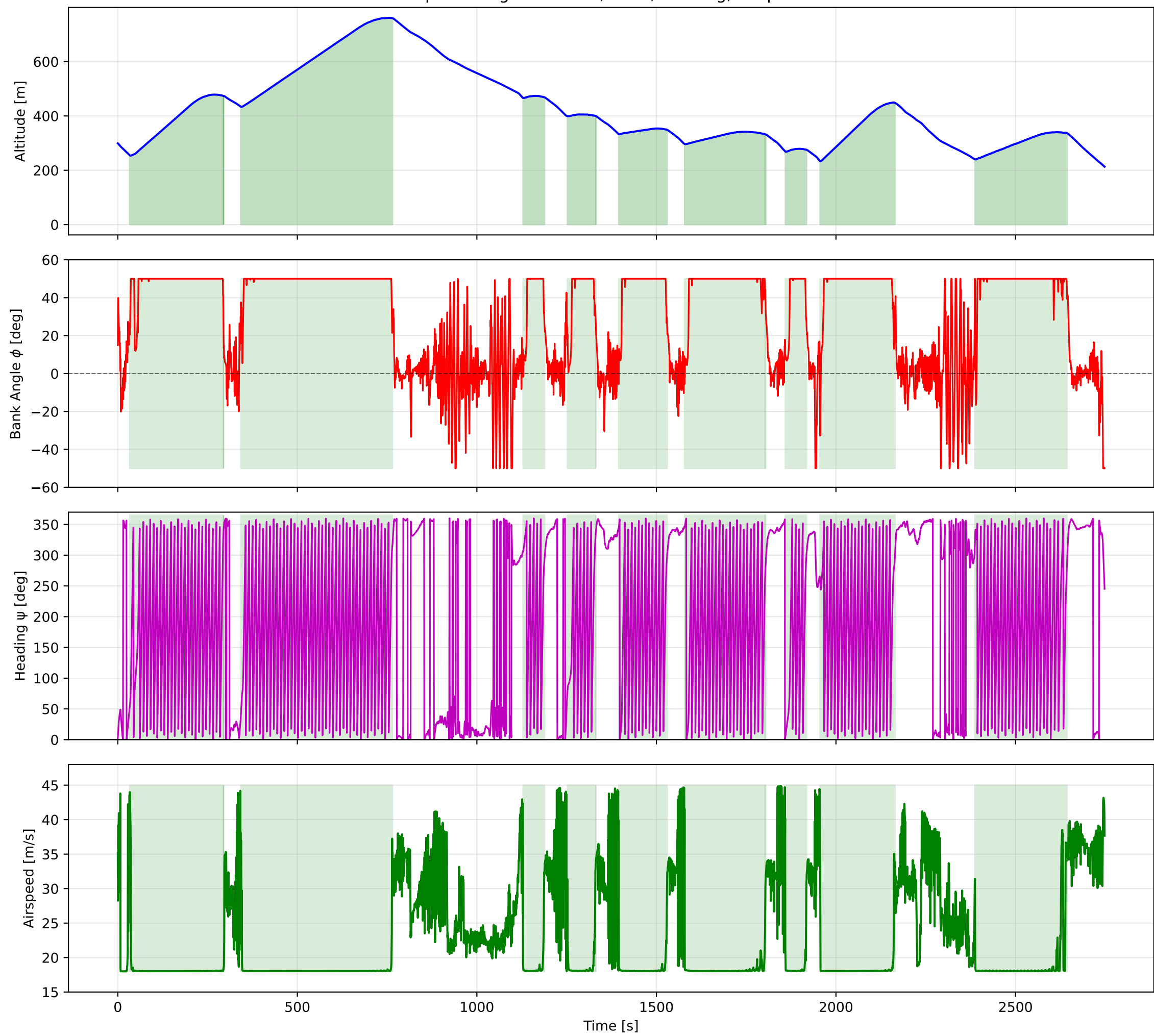
Episode flight: altitude, bank, heading, airspeed
