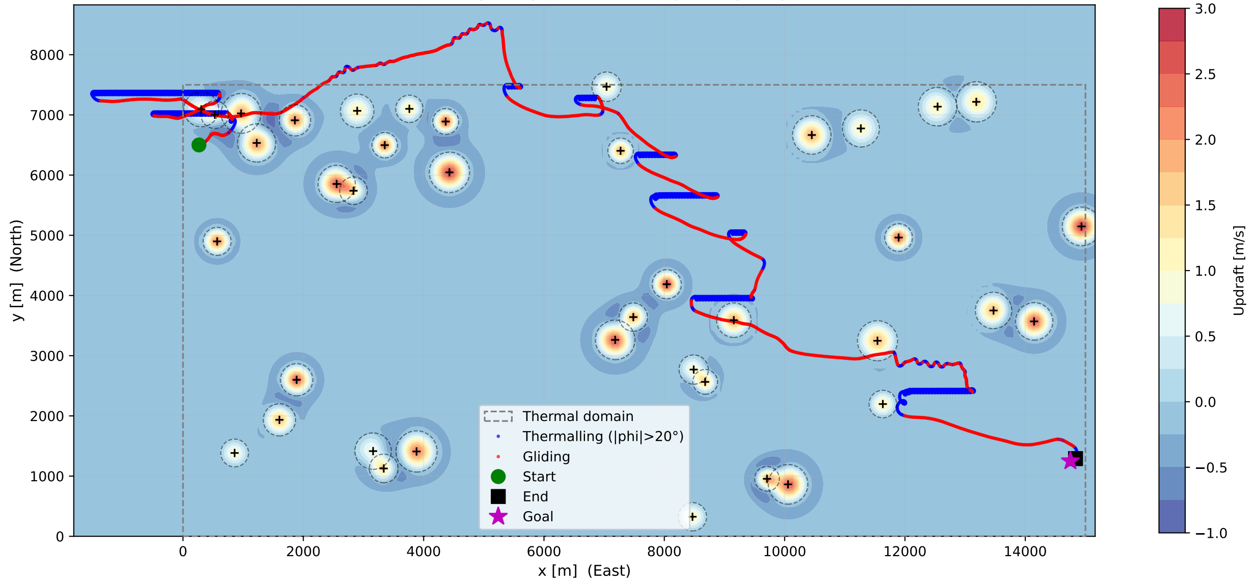
Climb-then-glide cycle: blue=circling, red=gliding
