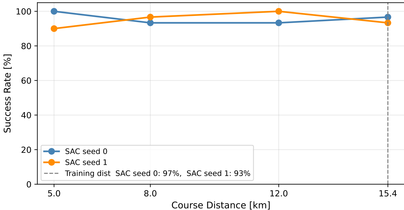
Generalisation: Course Distance
