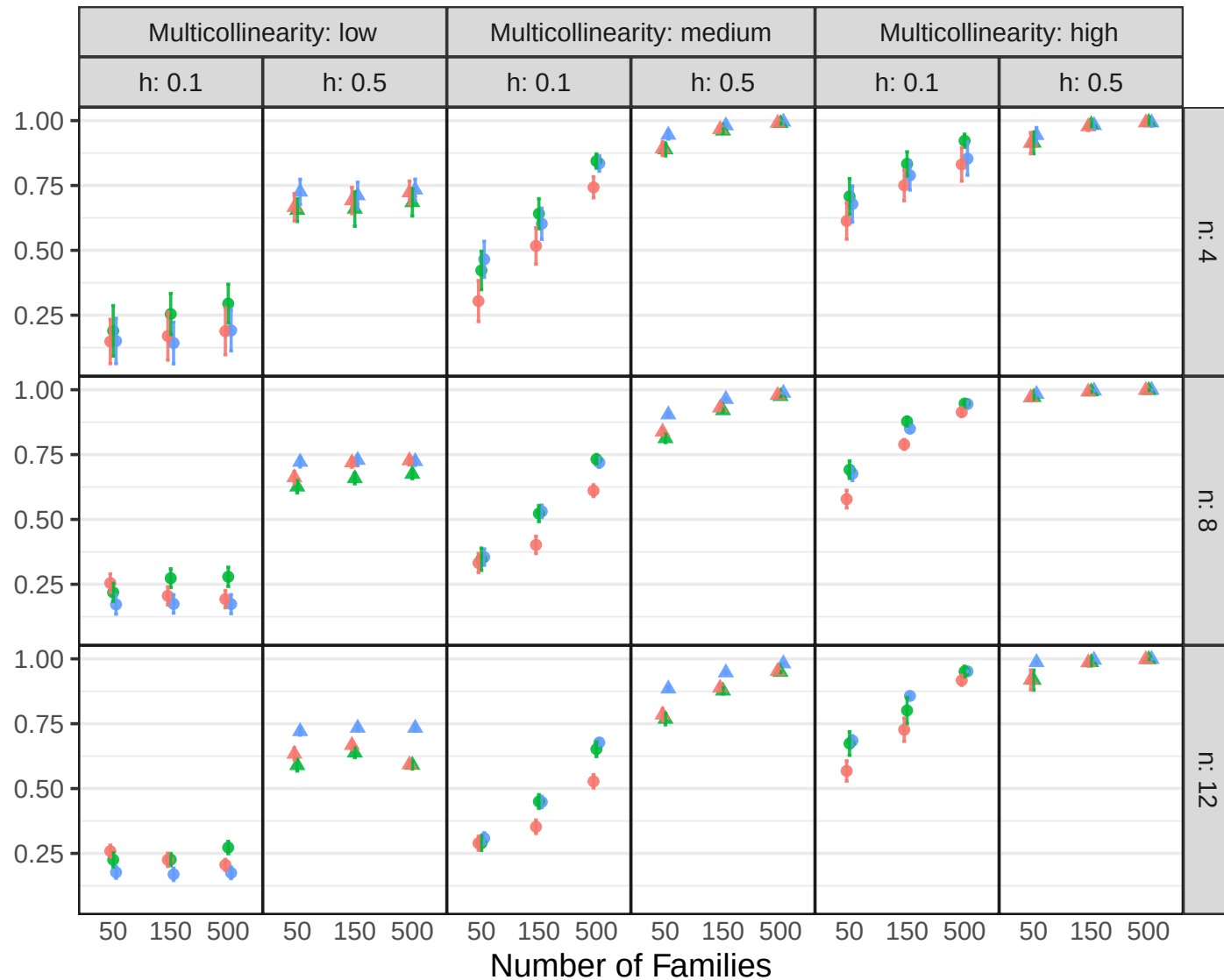
Pearson Correlation
