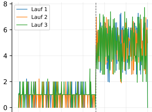
Isolation Forest
