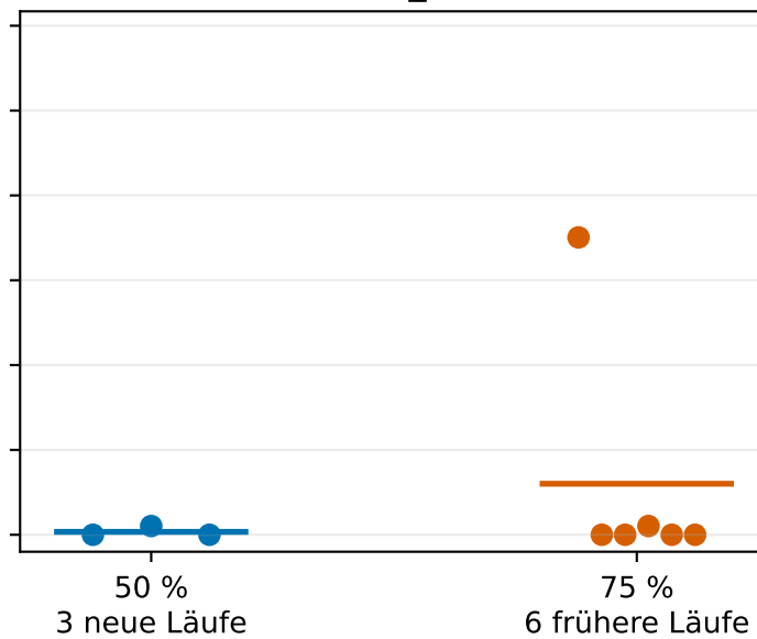
isolation_forest
