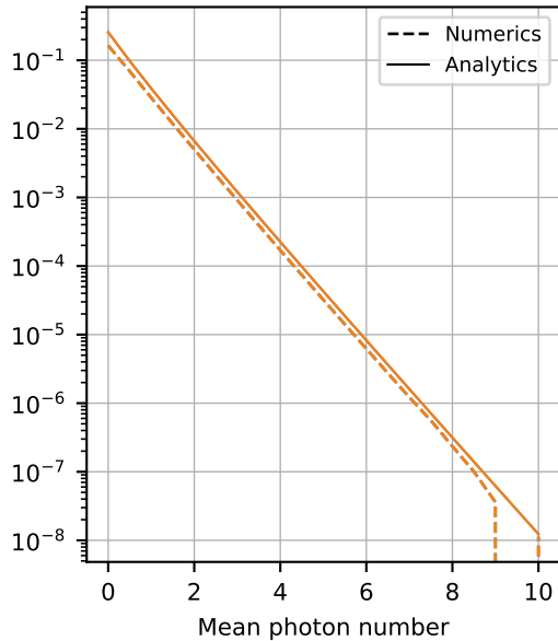
Logical fidelity
