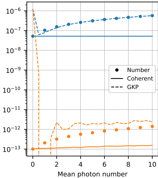
State fidelity
